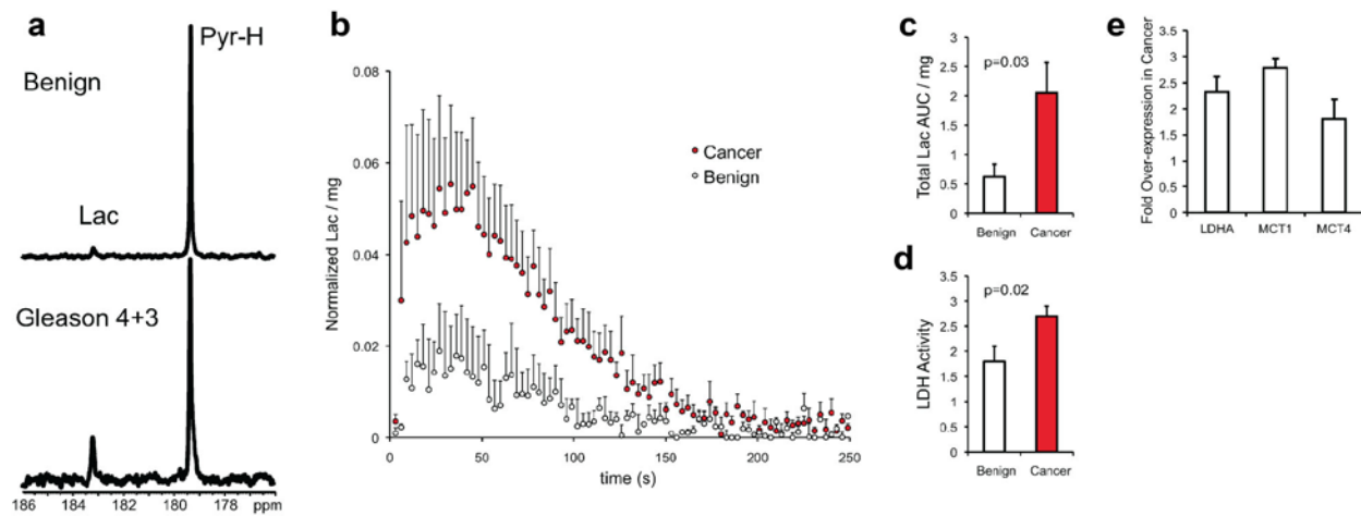
Fig. 4. a: A single spectrum taken at 90 sec post-injection of HP [ 1\text{-}^{13}\text{C} ] pyruvate in the bioreactor with benign (N = 4) or malignant TSCs (N = 4). b: Average HP Lactate dynamics for TSCs. c: Total normalized lactate area under the curve (AUC) and (d) LDH activity for benign And malignant TSCs. e: mRNA expression of lactate dehydrogenaseA (LDHA), monocarboxylate transporters1 (MCT1) and 4 (MCT4). All plots are represented as mean \pm SE.
