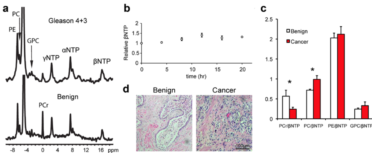
Fig. 3. a: 31 P spectra from living malignant and benign TSCs perfused in the MR-compatible bioreactor. b: Timecourse of \beta -NTP demonstrating preservation of ATP in the bioreactor. c: Ratios of metabolites to \beta -NTP in benign (N = 4) and malignant TSCs (N = 4). d: Representative H&E staining of TSCs post-perfusion in the bioreactor. PCr, phosphocreatine; PC, phosphocholine; PE, phosphoethanolamine; GPC, glycerophosphocholine; \alpha, \beta, \gamma -NTPs, nucleotide triphosphates. All ratios reported as mean \pm SE. P < 0.05.
