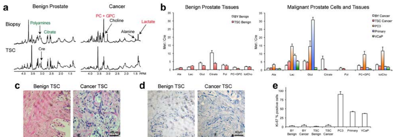
Fig. 2. a: Representative 1 H HR-MAS spectra from benign and malignant snap-frozen human biopsies and TSCs post-2 hr of culture. b: Quantified metabolite ratios for benign biopsies and TSCs (N = 16 and 14, respectively) as well as malignant BY and TSC (N = 12 and 9, respectively) compared to PC-3, primary prostate cancer cells and VCaP cells (all N = 4). c: Representative hematoxylin- and eosin- (H&E) staining and (d) Ki-67 immunohistochemistry of TSCs. e: Average percent positive Ki-67 staining of TSCs as compared to the other prostate tissues and cells. Ala, alanine; Lac, lactate; Glut, glutamate; Cre, creatine; Pol, polyamines; PC + GPC, combined phosphocholine and glycerophosphocholine; Tot Cho, total choline. All ratios reported as mean \pm SE.
