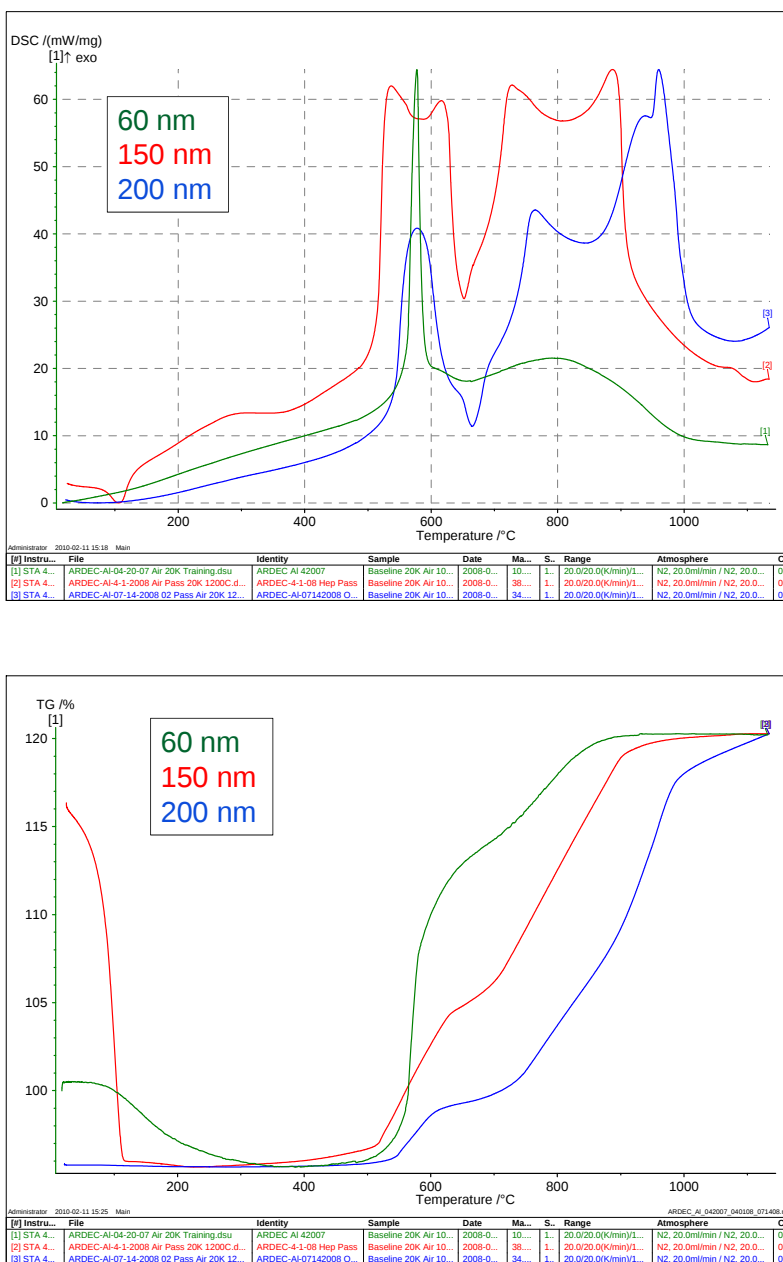
Figure 6 Results of DSC (top) and TGA (bottom) for three different particle size powders
