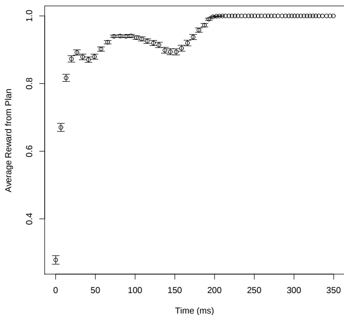
Average Reward per Time for c = \sqrt{4} for Random Large Scenario 2
