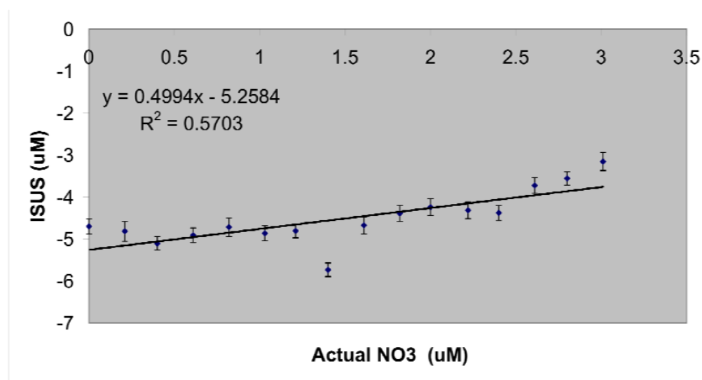
Figure 3: Results for laboratory calibration of ISUS 078. ISUS nitrate versus actual nitrate concentration (error bars are +/- 1SD for each sampling period)
