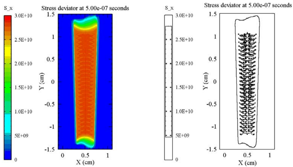
Figure 26 2D calculation of the high velocity impact of an aluminium target by aluminium flyer plate at impact velocity, U_0 = 382 \text{ m/s} - shear stress and the same plot processed graphically
