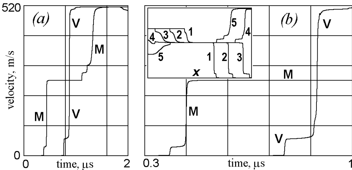
Figure 12 One-dimensional calculation of the high-velocity impact of an aluminium target by a steel flyer plate at impact velocity, U_0 = 365 \text{ m/s} using the in-house ALE code. The velocity-time profiles M in the middle of the target are plotted along with the profiles V at the free surface of the target. Velocity profiles inside the flyer plate-target assembly are drawn in the insert of the graph (b) at every 0.25 \mu\text{s} of the profile evolution.
