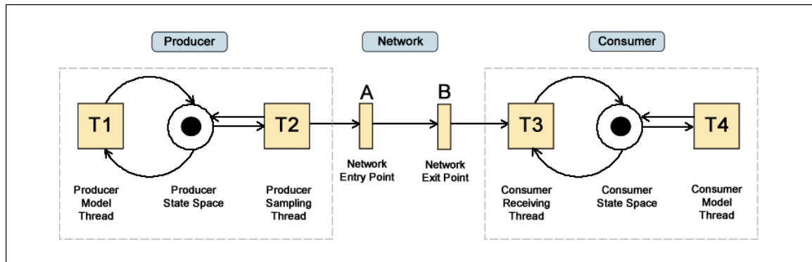
Figure 4: Multithreaded Architecture.
