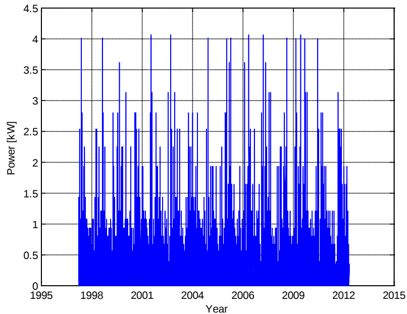
Figure 10. Power vs. time.
