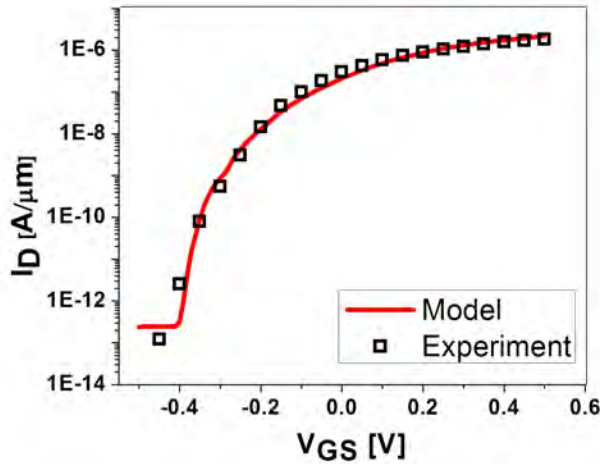
Figure 3.2: Measured experimental and simulated I_{\text{D}}\text{-}V_{\text{GS}} data.
