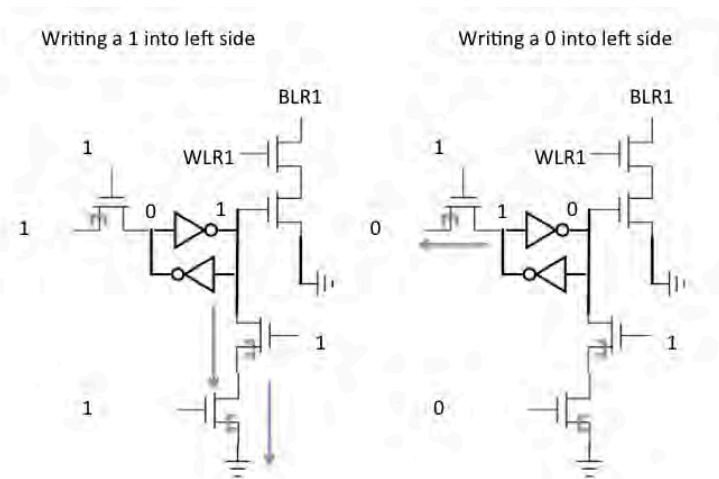
Figure 5.10: Two-sided Register File write operations.
