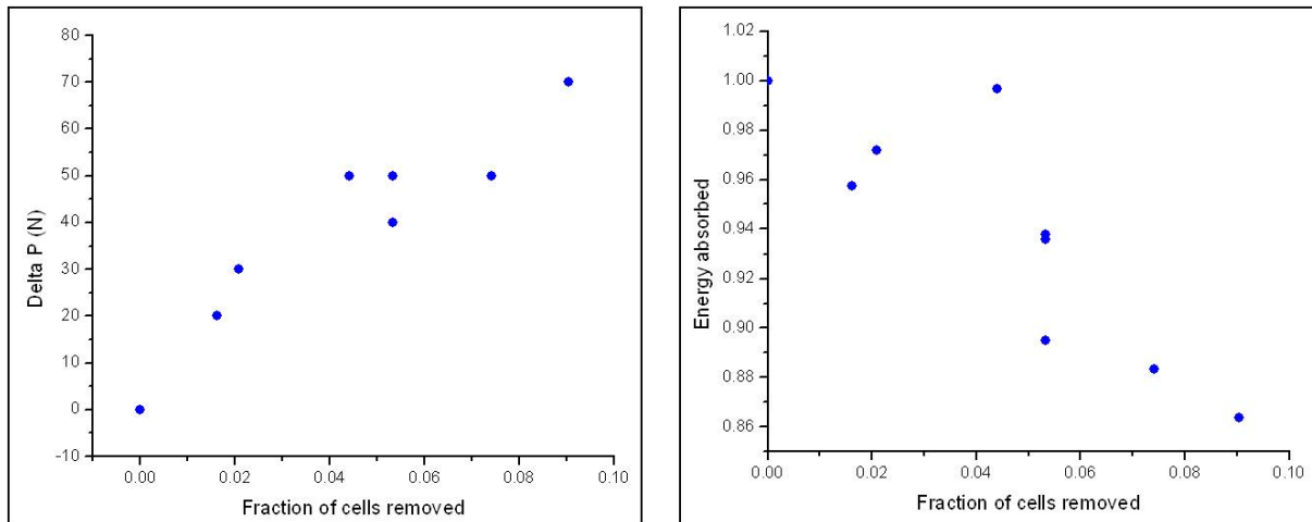
Figure 2.4: Influence of fraction of cells removed on \delta P and energy absorbed
