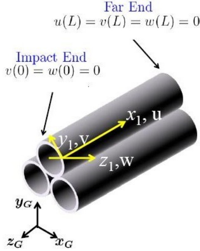
Figure 3.16: Diagram showing the boundary conditions used on the honeycomb during eigenbuckling analysis. These boundary conditions are also used for crush simulations. x_1 , y_1 and z_1 are the local shell co-ordinates on a single cell corresponding to axial ( u ), circumferential ( v ) and radial ( w ) displacements. x_G , y_G and z_G are the global co-ordinates for the model.
