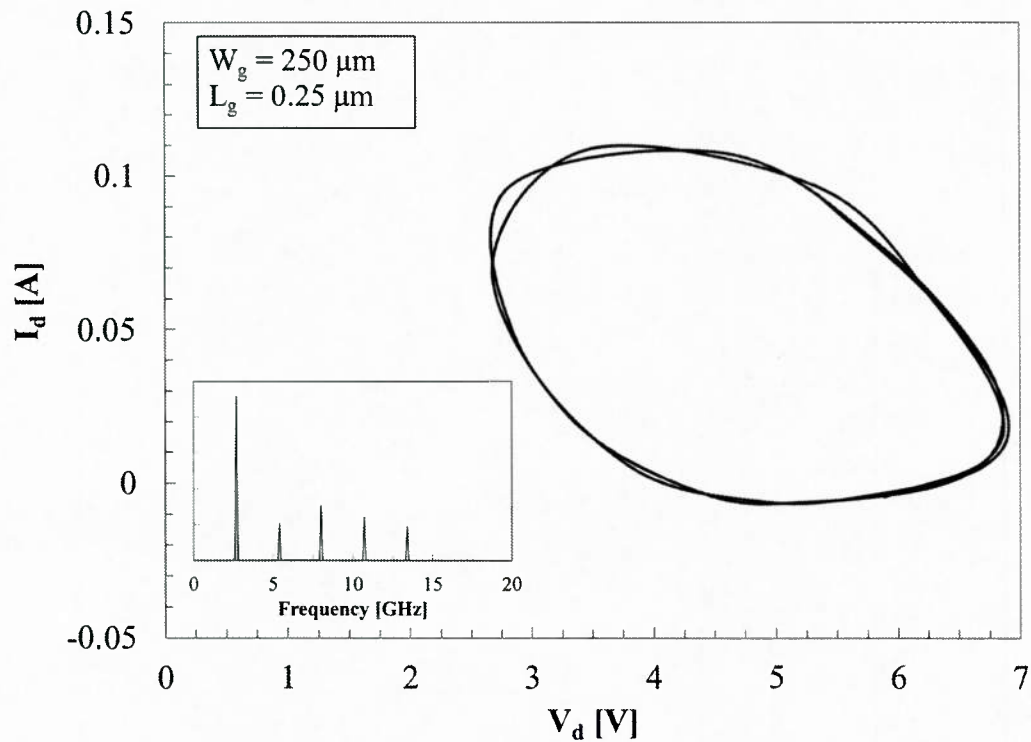
Figure 6. Loadline of a 0.25 by 250 \mu\text{m} device at 5 V drain bias and load impedance of 58.5 - 12.2i \Omega , with P_{in} = 23 dBm.
