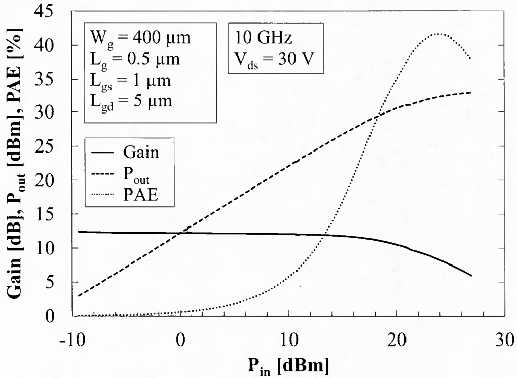
Figure 2. Typical 10 GHz load pull power sweep at 30 V of drain bias of a 0.5 by 400 \mu\text{m} device.
