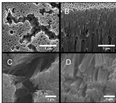
Figure 123. The SEM images show bundles of ssq channels inside the anodisc alumina membrane (AAM) pores
