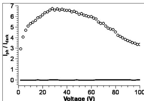
Figure 96. Ratio of photocurrent ( I_{ph} ) under 100 μW illumination at 900 nm to dark current ( I_{dark} ) for PbS-OLA (line) and PbS-DT (open circles) thin films.
