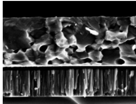
Figure 116. 1- \mu\text{m} Thick \text{CuInS}_2 Film from Aqueous Precursor
