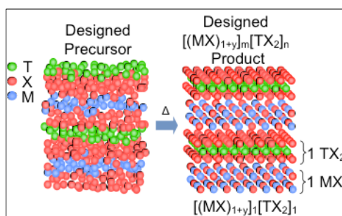
Figure 102: A schematic of a precursor designed to form [(MSe)_{1+y}]_1(TSe_2)_1 .
