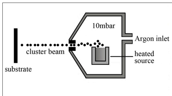
Figure 84. The self-assembly fabrication process.
