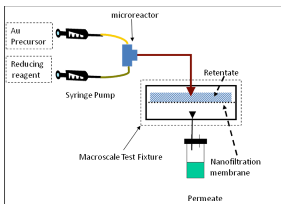
Figure 59. Fluidic control schematic for in-line microreactor and nanofiltration. The output flow (total flow rate: 0.08 mL/min) of the microreactor was introduced directly to the MTF equipped with a membrane.
