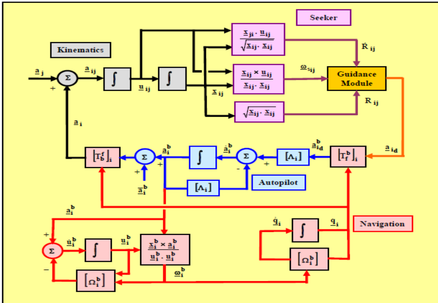
Figure A.1: Intelligent Integrated Navigation, Guidance &amp; Control Test Bed
