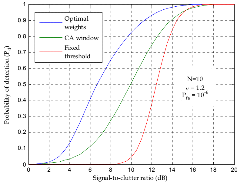
Figure 15: ROC comparison between the fixed-threshold and the adaptive thresholds determined by the optimal weights and a CA window with L = 8 for the spatially correlated K -distributed clutter with the correlation given by (40) and (41).
