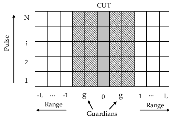
Figure A1: Using neighbouring cells to estimate CUT (the case of multi-look in pulse and multi-look in range).
