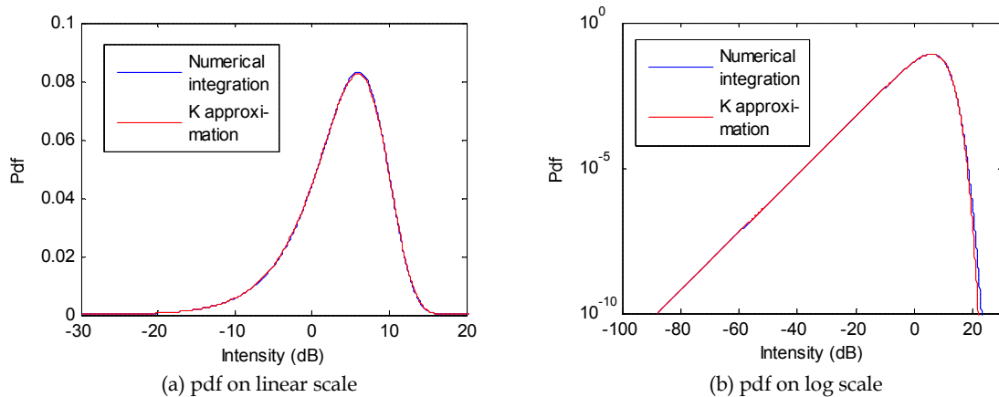
Figure 17: Pdf comparison between numerically integrated (viewed as 'true distribution') and the K approximation ( \nu = 1.0 , \mu = 1.0 and SCR = 5dB ) The shape parameter \nu_1 is determined by (B18).
