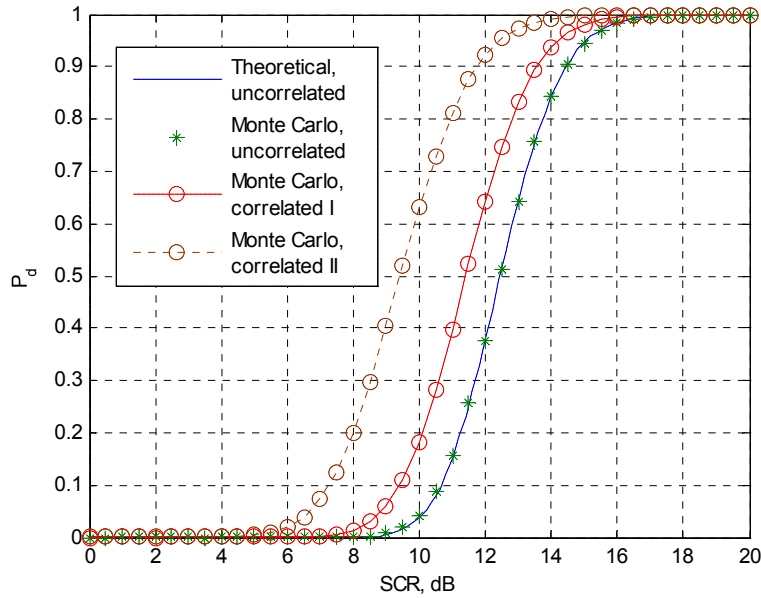
Figure 10: ROC comparison between uncorrelated and correlated K -distributed clutter embedded with uncorrelated Gaussian target signals. Two correlated cases are shown: Case I with correlation coefficients of \rho_n = \exp(-n) , n = 0, \dots, N-1 , and Case II with correlation coefficients of \rho_n = \exp(-n) , n = 0, \dots, N-1 ( P_{fa} = 10^{-6} , \mu = 1 , \nu = 1.2 and N = 10 ).
