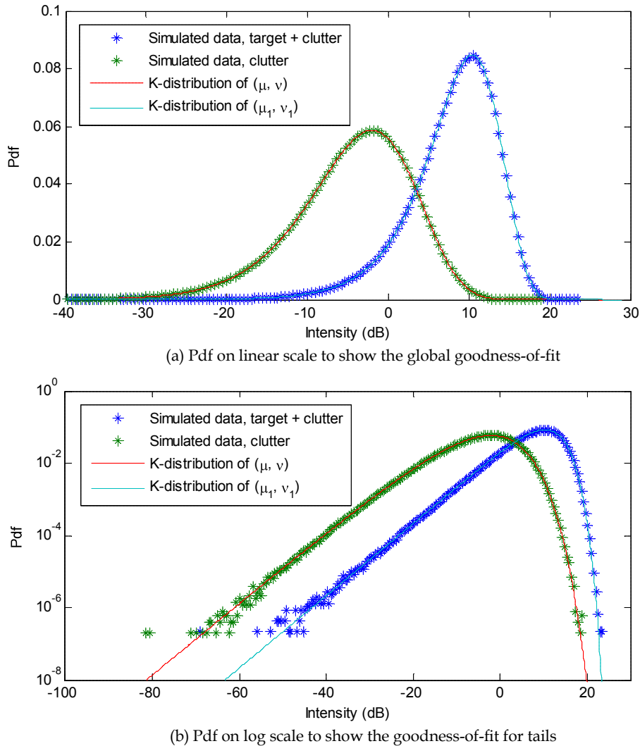
Figure 19: Goodness-of-fit for distribution of Gaussian target embedded in K-distributed clutter ( \mu = 1.0 , \nu = 1.2 , SCR = 10dB ).
