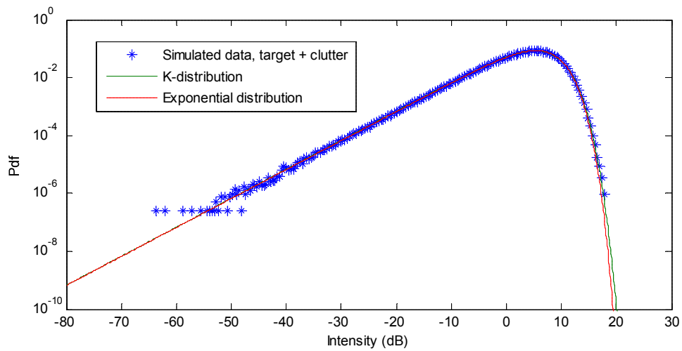
Figure 21: Goodness-of-fit for distribution of Gaussian target embedded in K-distributed clutter ( \mu = 1.0 , \nu = 5.0 , SCR = 4dB ). The approximated K-distribution is almost identical to the exponential distribution.
