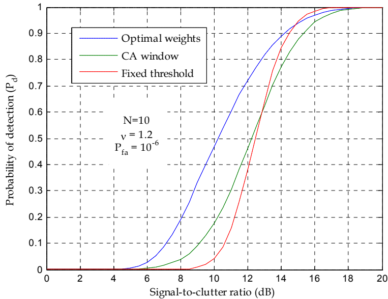
Figure 16: ROC comparison between the fixed-threshold and the adaptive thresholds determined by the optimal weights and a CA window with L=8 for the spatially correlated K -distributed clutter with the correlation given by (43) and (41).
