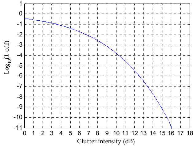
Figure 3: Cdf of multi-look K -distributed clutter shown as \log_{10}(1 - cdf) ( \nu = 1.2 , \mu = 1.0 , N = 10 ).
