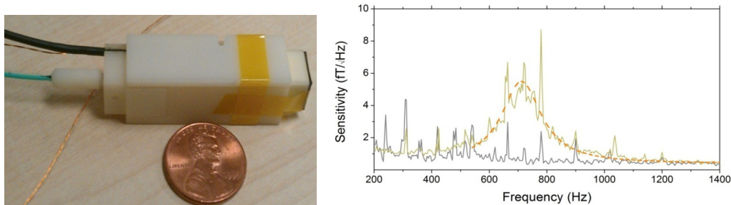
Figure 1. Left: Miniaturized scalar atomic magnetometer; Right: Experimentally measured RF magnetometer sensitivity. (Green line): Magnetometer tuned to 720 Hz resonant frequency. (Black line): Magnetometer tuned to a very high frequency (not shown on the graph). The black line serves as the reference noise floor of the sensor. The hump at 720 Hz is mostly likely due to the magnetic Johnson noise inside the shields created by thermal eddy currents in mu-metal.
