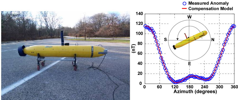
Figure 5. Example of the azimuthal response (blue circles) of an UUV produced by systematically spinning the vehicle 360 degrees through the Earth's field. A standard compensation model (red curve) was applied to fit the response with a high degree of accuracy.
