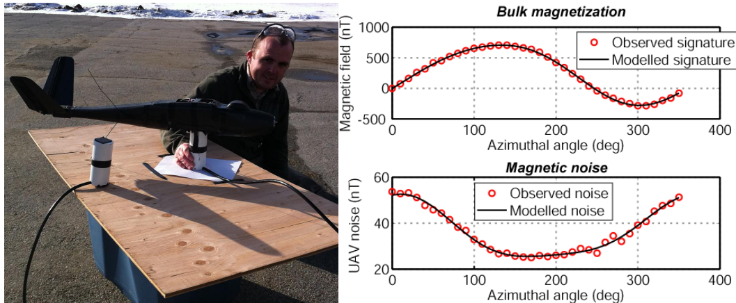
Figure 6. Left: Photograph of the Vertek Nighthawk UAV being utilized for preliminary magnetic signature tests. Right: Observed and predicted bulk magnetic signature and noise variation as a function of azimuth. The bulk magnetization contains both induced and permanent effects.
