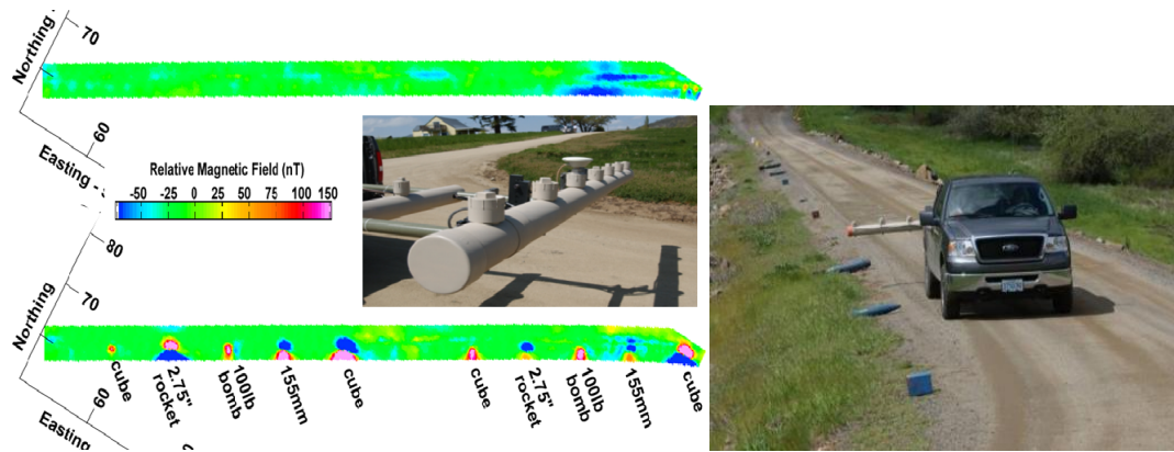
Figure 3. Left: Change detection map pairing - top figure shows the magnetic field anomaly experienced during a background pass and the bottom figure shows the map after IED surrogates were emplaced. Right: The magnetic field change detection platform mounted in the bed of a pick-up truck.
