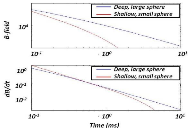
Figure 4. Effective sensitivity of B and dB/dt sensor modalities. At late times after cessation of the primary field discrimination of large/deep objects from small/shallow ones is more readily observed in B than in dB/dt simulated data.
