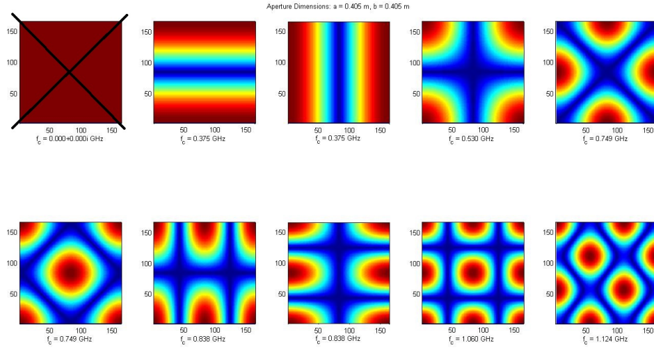
Figure 4.14: First 10 TE^z approximated modes, square aperture, N = 165
