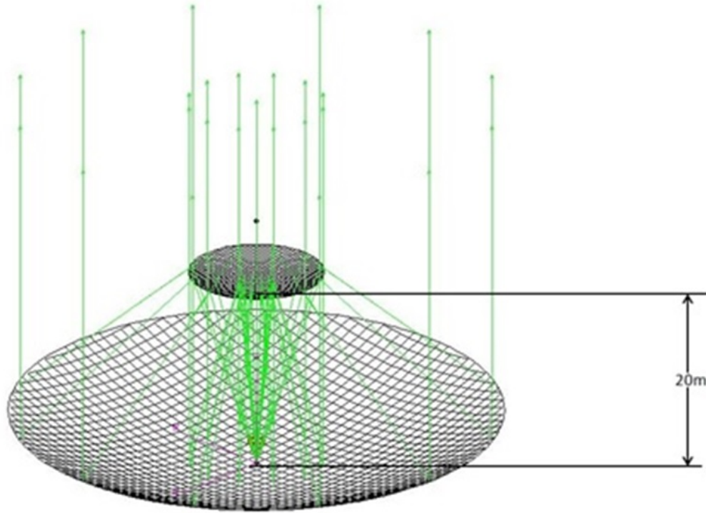
Figure 4.11: Wire frame view of the 50 meter diameter circular, parabolically contoured reflector used as the baseline antenna system for the sparse reflector. Graphic generated using SatCom TM
