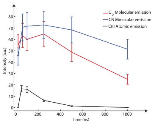
Figure 28. Spatially integrated temporal emission profile from atomic and molecular plasma species resulting from filament-induced ablation of graphite.
