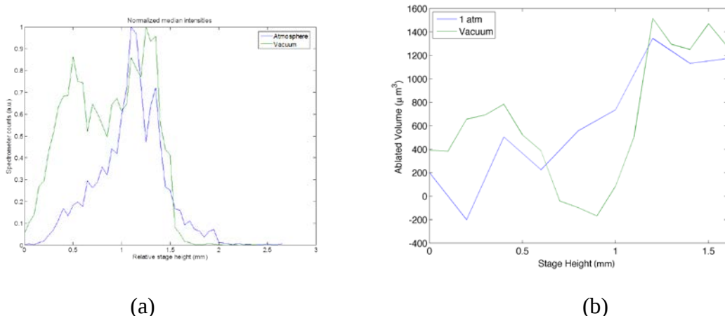
Figure 11: (a) Comparison of LIBS signal intensity of the 288.16 nm Si line in vacuum and open atmosphere as a function of sample location for a spherical lens (laser focus at \sim 0.9 mm) . (b) Plot of the ablated volume corresponding to the data in (a).
