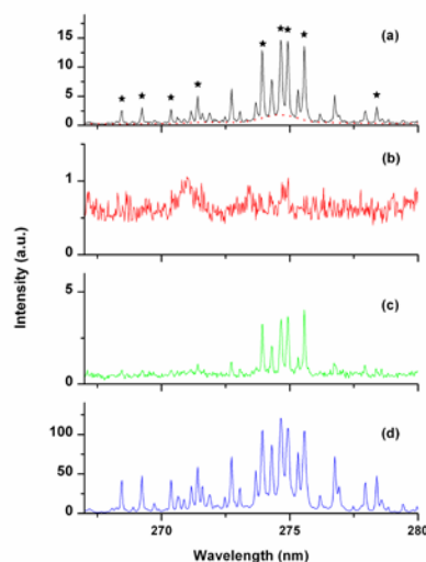
Figure 46. LIBS spectra of iron from a) a single Nd:YAG pulse, b) a single CO 2 laser pulse, c) double pulse spectra with CO 2 following Nd:YAG by 1 \mu\text{s} compared with Nd:YAG alone LIBS spectrum and d) double pulse spectra with CO 2 preceding Nd:YAG by 1 \mu\text{s} . (Acquisition delay: 1 \mu\text{s} , duration of acquisition: 25 ns). In a), the dotted line shows a background spline interpolation and the stars indicate the lines used for plasma temperature calculation. Baseline correction is applied for all spectra.
