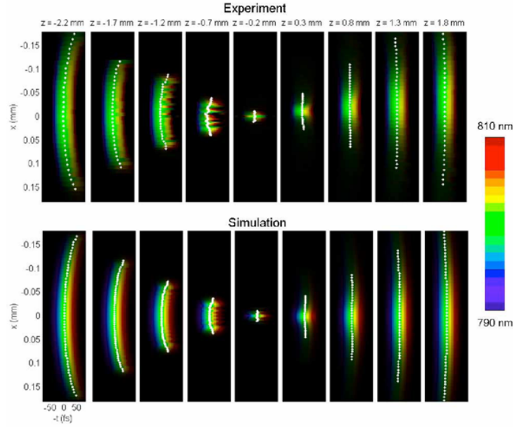
Figure 6: E(x,z,t) in the focal region the spatial profile that are particularly visible at z = -0.7\text{ mm} . 1 These hot spots in the electric field intensities cause localized nonlinear effects on the target surface since the intensity is the square of these electric fields of a plano-convex lens. The spherical aberrations introduced by this lens result in ripples in the electric field intensities.
