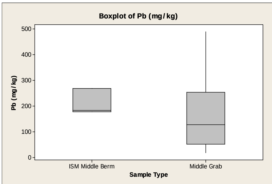
G-1.3. Boxplots of “Middle Grab” and “ISM Middle Berm”
