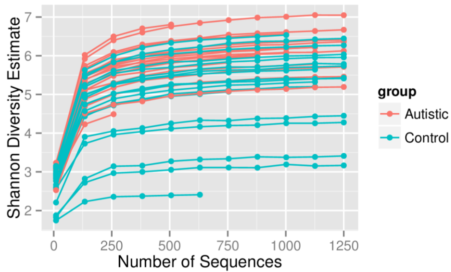
(a) Rarefaction curves for the Shannondiversity estimate
