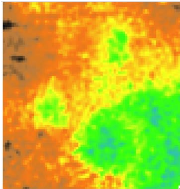
Figure 2. Sample DEM.
