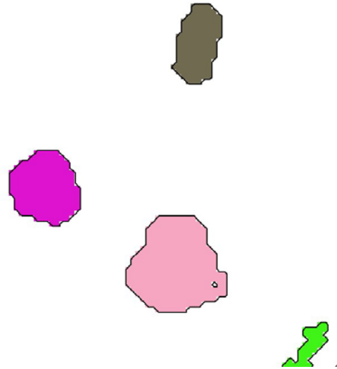
Figure 5. Selected ponds.
