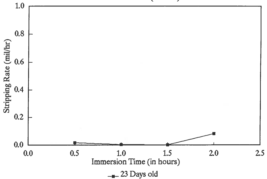
Pure Nickel (N-100)
