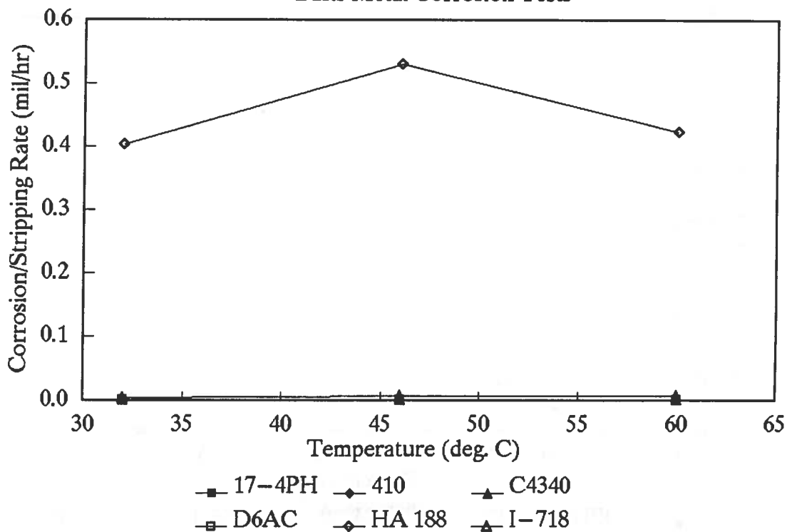
Basis Metal Corrosion Tests
