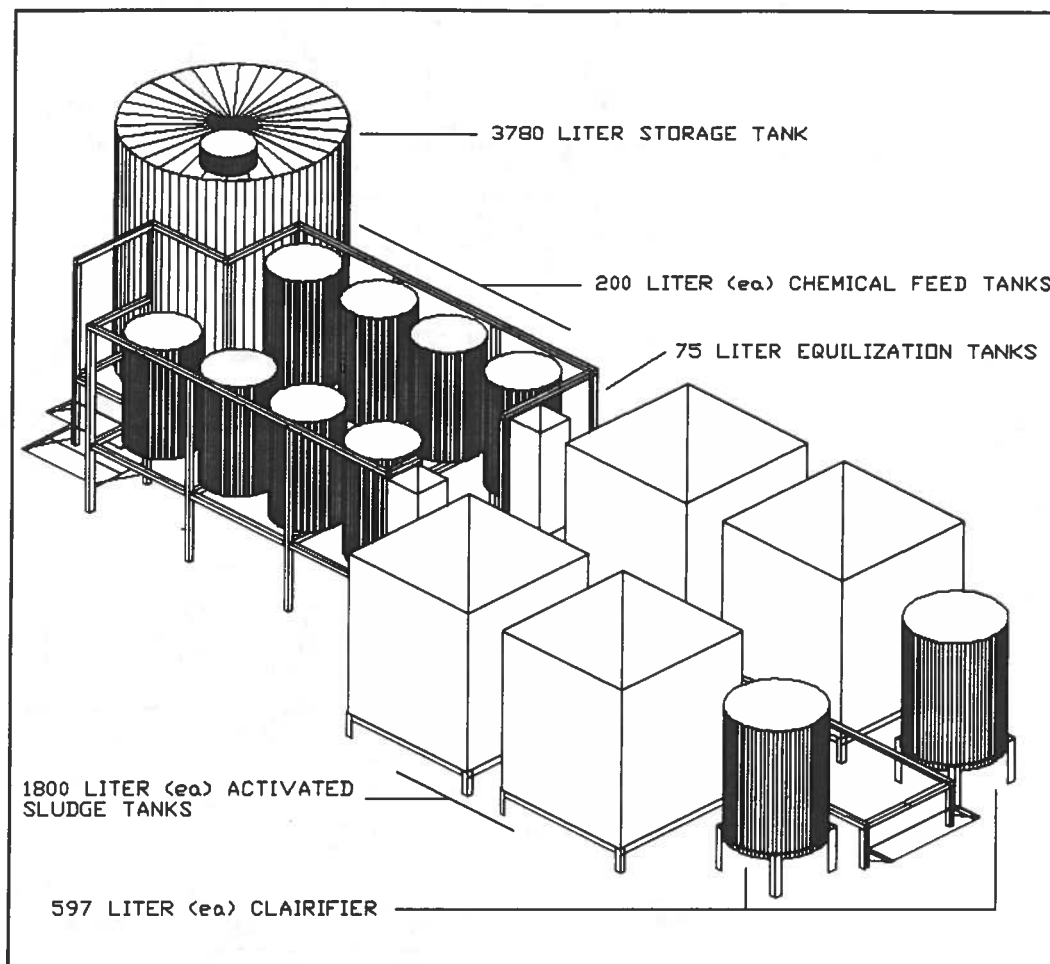
Figure 1. Pilot-Plant Design.
