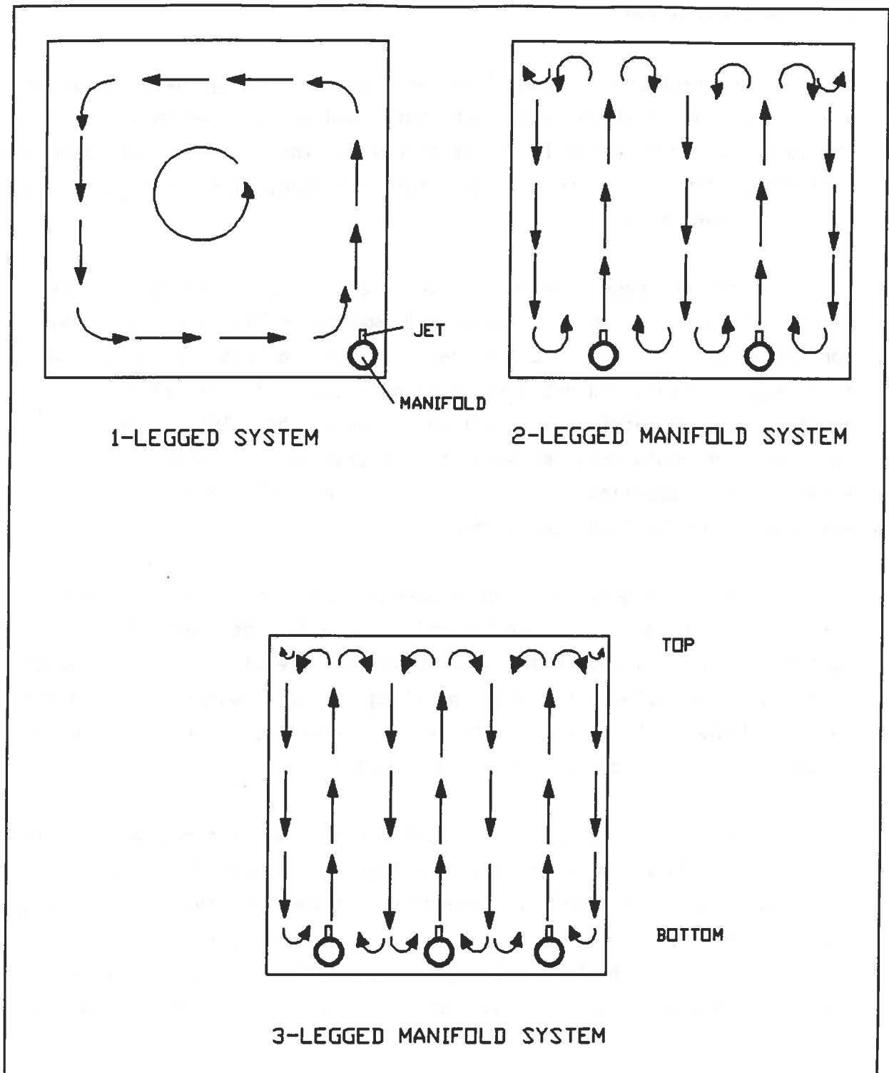
Figure 7. Current Flow for 1-, 2-, and 3-legged Manifold Systems.
