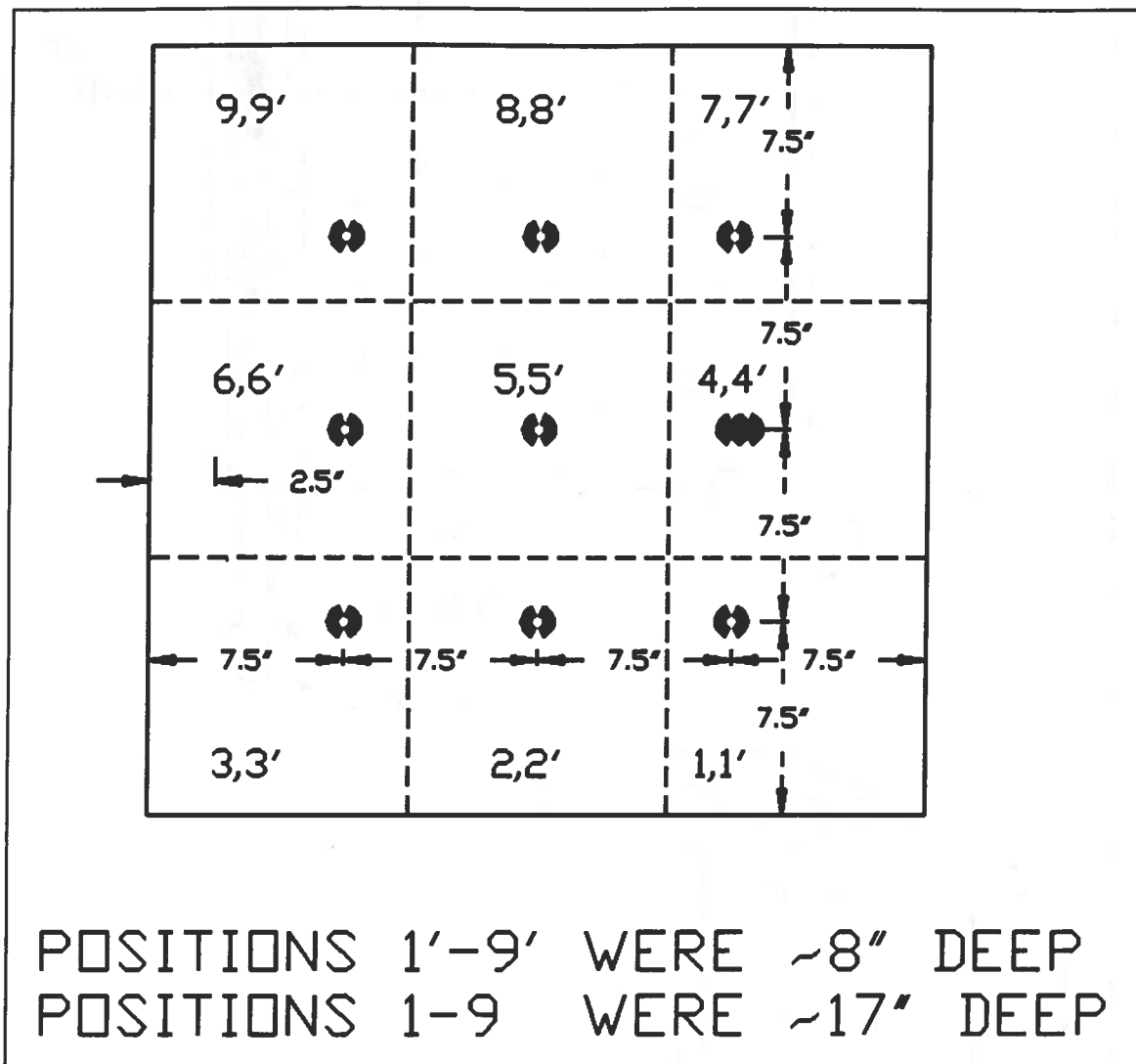
Figure 6. Fluid Agitation Test Placement of Candies.
