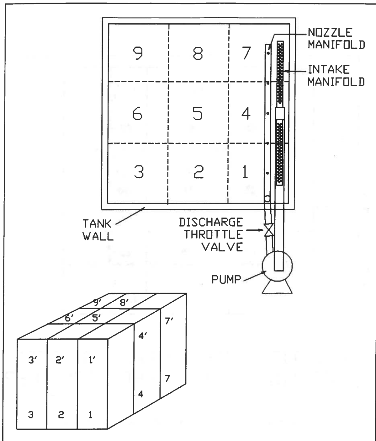
Figure 5. Fluid Agitation Test Equipment Layout.
