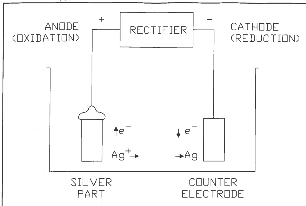
Figure 4. Electrolytic Stripping Reactions.
