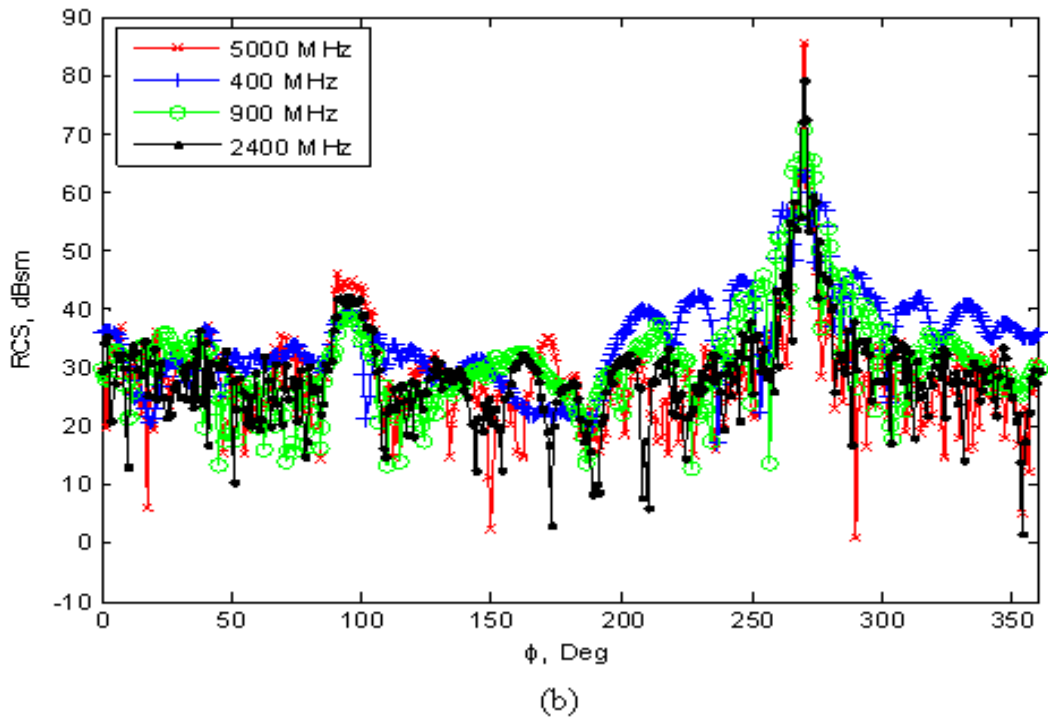
Figure 17. Comparison between four frequencies of azimuth bistatic co-polarized RCS of the horizontal axis wind turbine with fiberglass blades for an incident wave from the side ( \theta = 90^\circ , \theta_i = 90^\circ , \phi_i = 90^\circ ): (a) \sigma_{\theta\theta} , (b) \sigma_{\phi\phi} .
