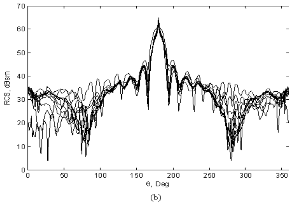
Figure 19. Azimuth bistatic co-polarized RCS for a collection of blade angles from 0^\circ to 120^\circ in ten degree increments, front incidence ( \theta = 90^\circ , \theta_i = 90^\circ , \phi_i = 0^\circ ), fiberglass blades, 400 MHz: (a) \sigma_{\theta\theta} , (b) \sigma_{\phi\phi} .
