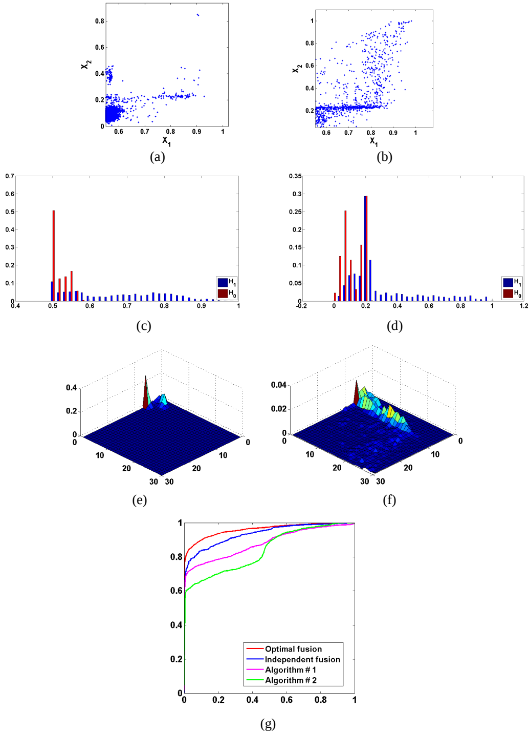
Figure 11. Example of detecting white plane class. Algorithms 1 is using modified Hausdorff distance metrics on bispectral features, and algorithm 2 is using SVM on spectral features. (a) and (b): The local confidence values of the two algorithms. (c) and (d): The distribution of local outputs under each hypothesis. (e) and (f): The joint probability density function of the local outputs under H_0 and H_1 . (g): The ROC curves of the individual algorithms and the two fusion processors.
