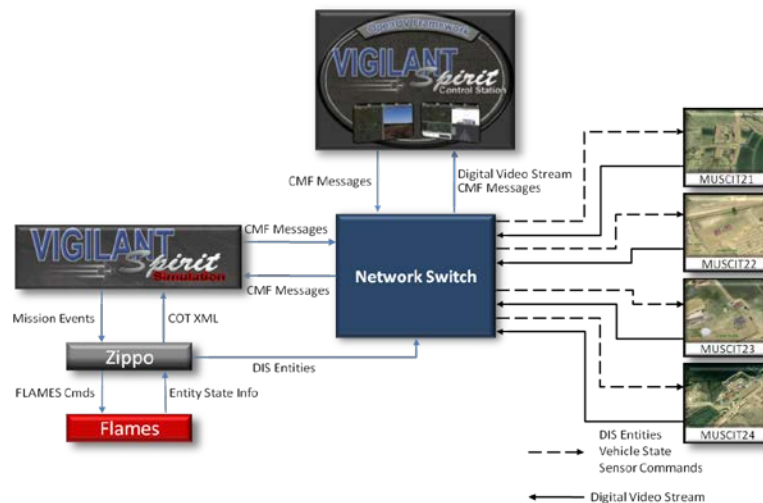
Figure 1. Illustrated architecture for the MUSCIT Spiral 3 Simulation
