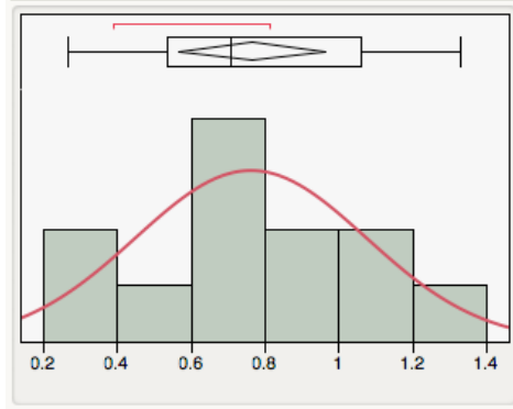
Figure 27. Freeze-Wet Taxiway PCC (with outliers removed)
