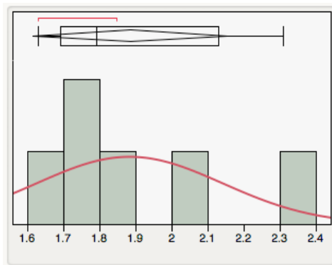
Figure 29. Freeze-Wet Taxiway AC/AAC (with outliers removed)
