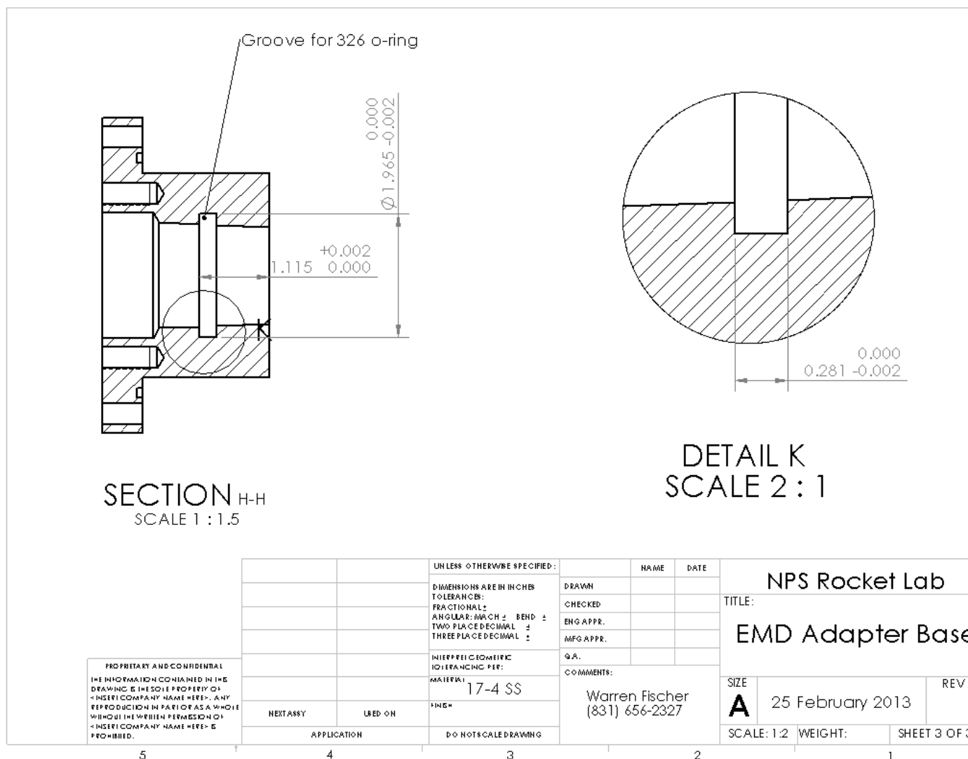
Figure 41. EMD Injector Adapter Fabrication Drawing (Page 3 of 3)
