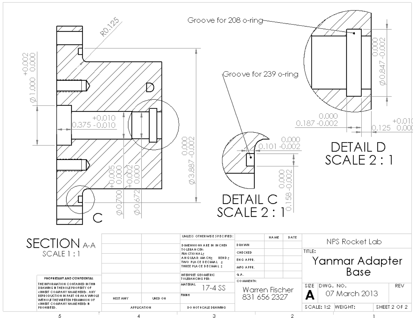
Figure 36. Yanmar Injector Adapter Fabrication Drawing (View 2 of 2)
