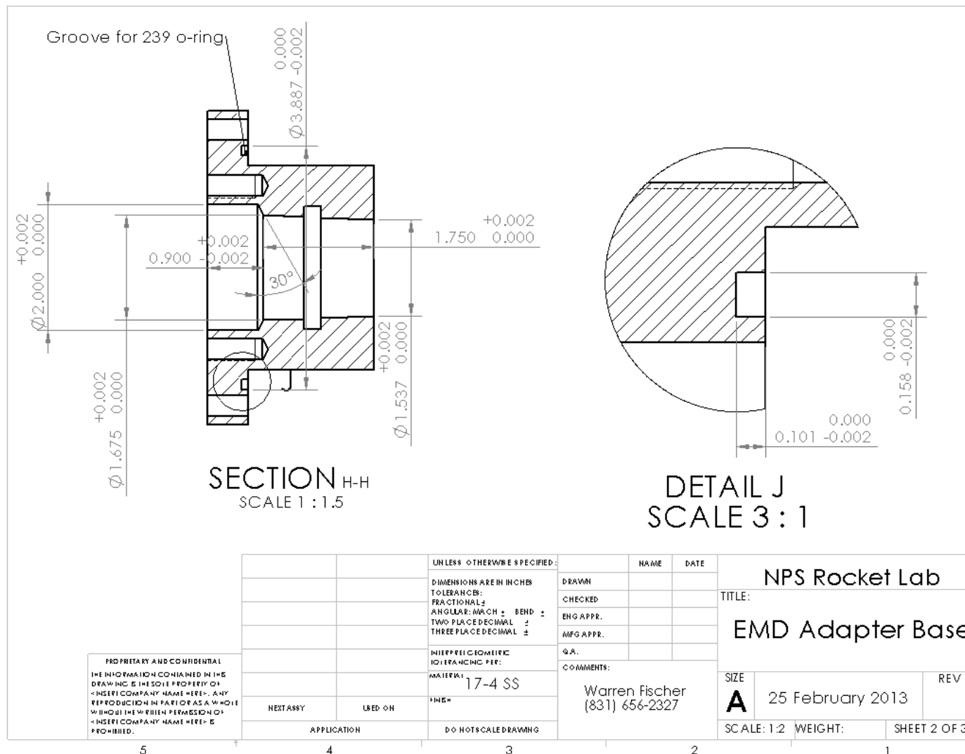
Figure 40. EMD Injector Adapter Fabrication Drawing (Page 2 of 3)
