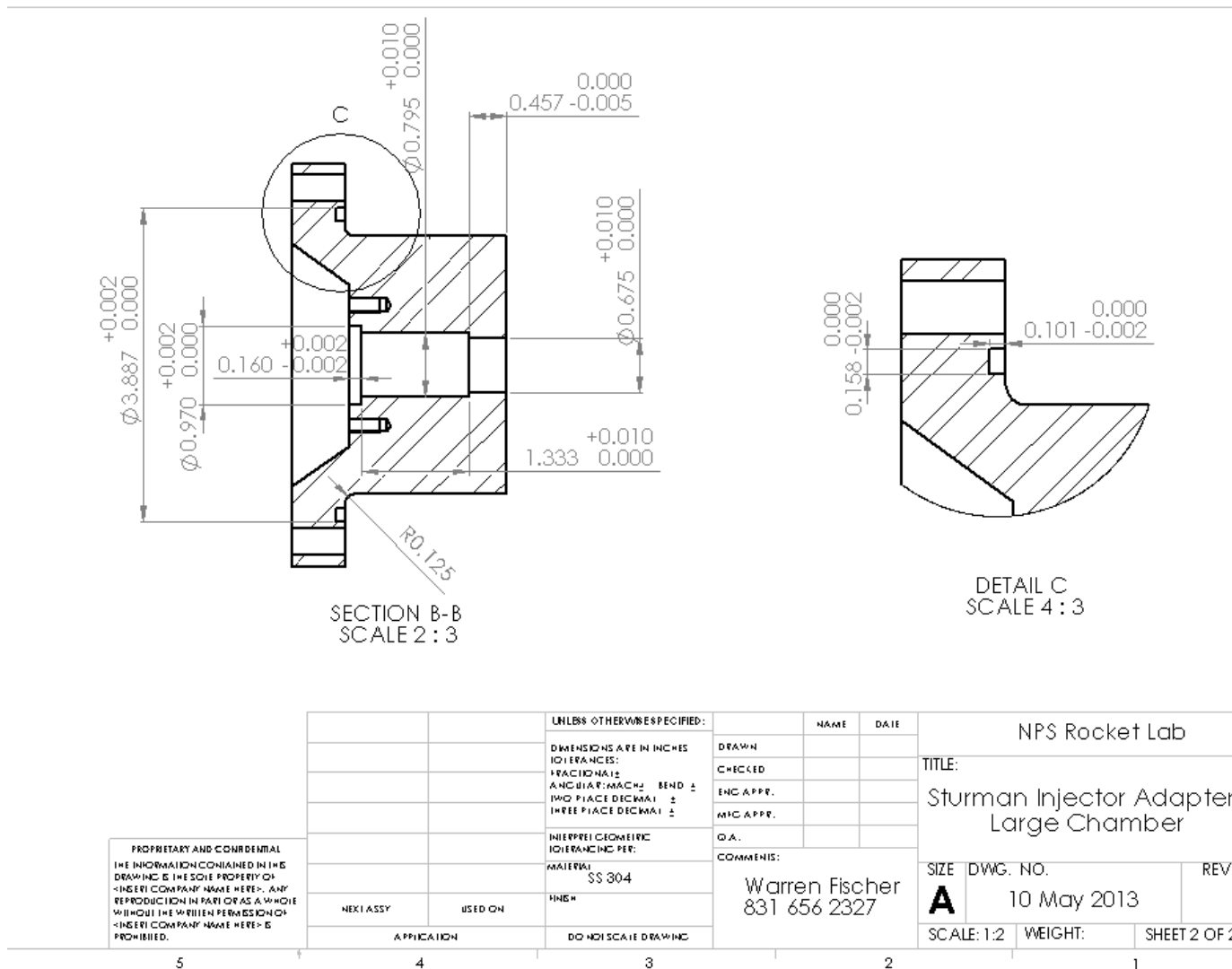
Figure 33. Sturman Injector Adapter Fabrication Drawing (Page 2 of 2)
