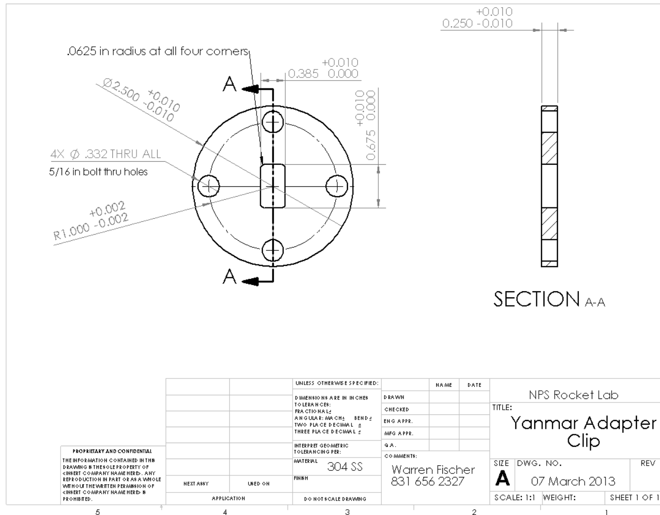
Figure 38. Yanmar Injector Adapter Clip Fabrication Drawing
