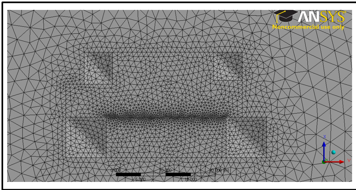
Figure 9. Mesh for ANSYS CFX analysis.
