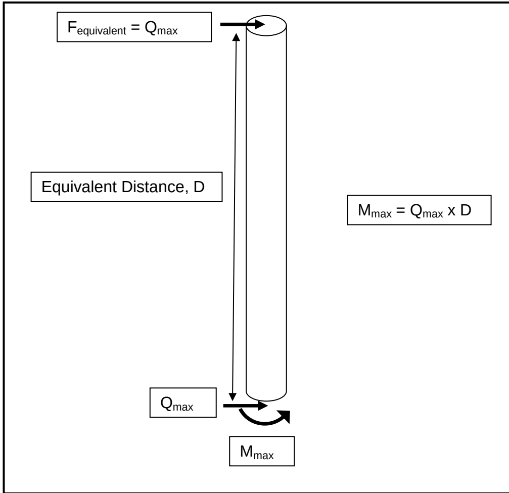
Figure 44. Equivalent force diagram.
