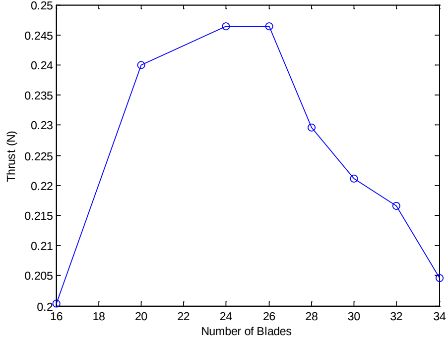
Figure 22. Thrust as a function of the number of blades at 8,000 RPM.
