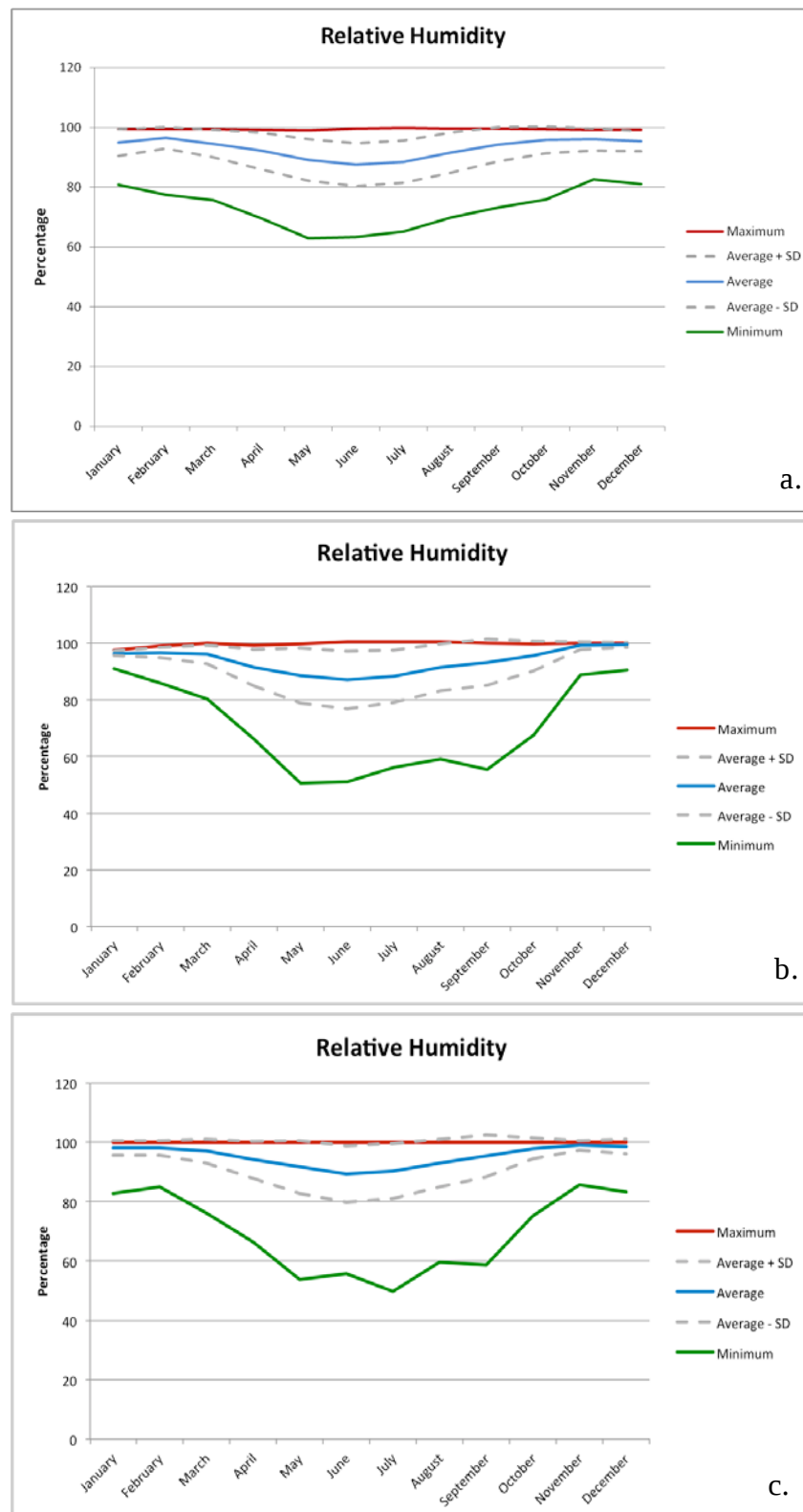
Figure 6. Relative humidity at target sites (a) Crawford Point, 1995–2010; (b) NASA-SE, 1998–2012; and (c) Saddle, 1997–2009.
