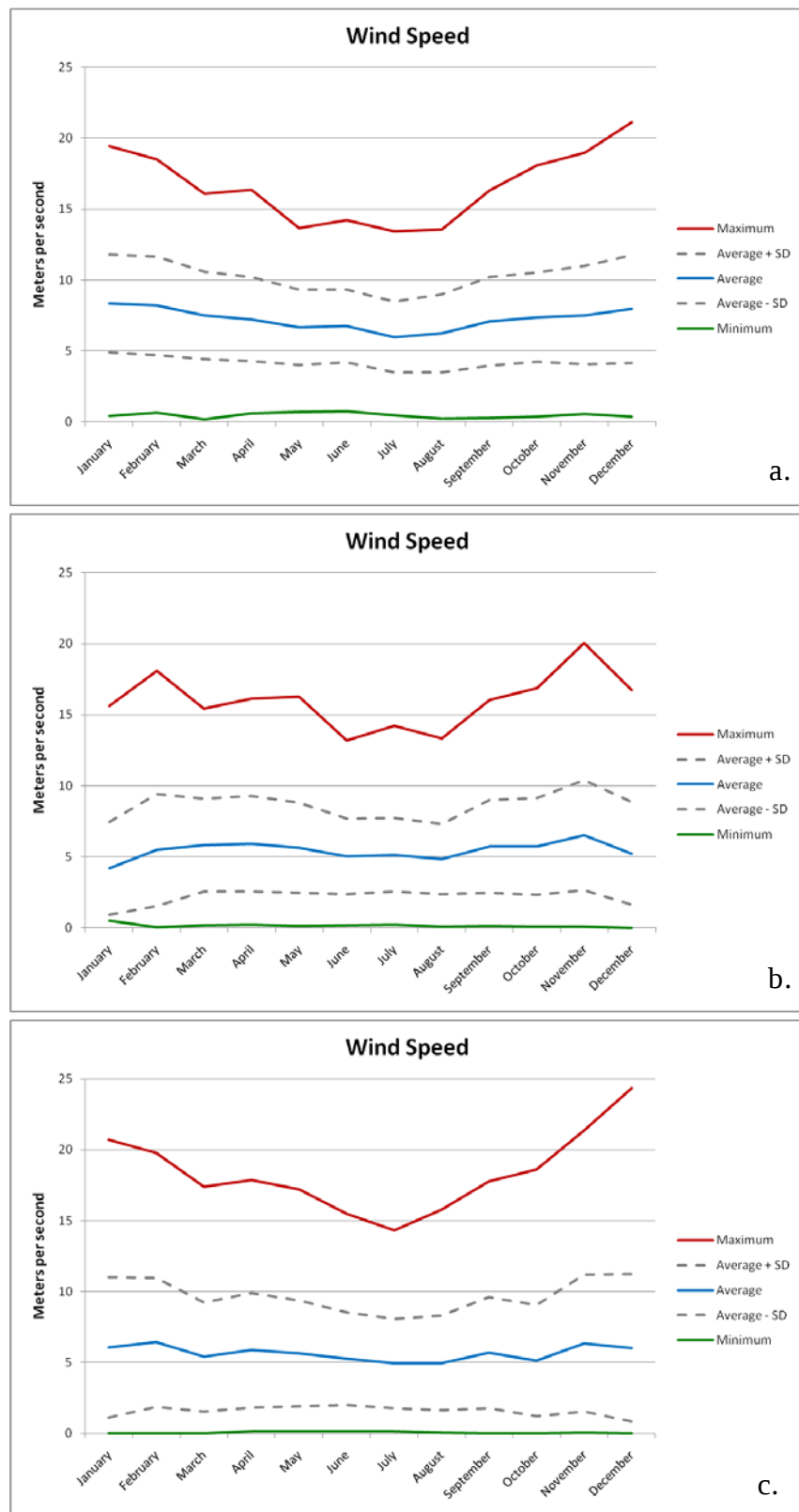
Figure 4. Wind speed at target sites (a) Crawford Point, 1995–2010; (b) NASA-SE, 1998–2012; and (c) Saddle, 1997–2009.
