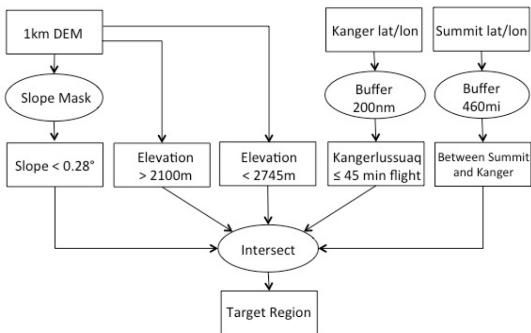
Figure 1. Methodology flowchart.
