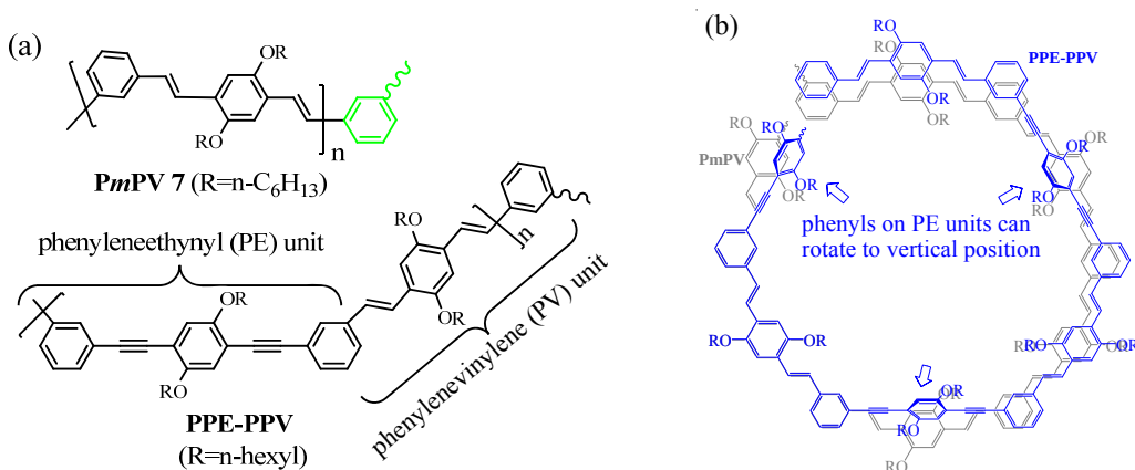
Scheme 3. (a) Chemical structures of PmPV and PPE-PPV. (b) Overlay of PmPV (grey color) and PPE-PPV (blue color) oligomers in helical conformations, showing that the PPE-PPV has a slightly larger conformation cavity. The thick arrows point to the phenyl groups that can rotate to vertical position.
