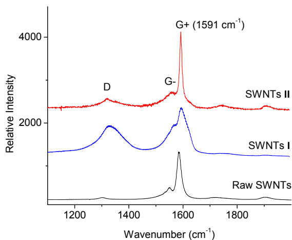
Figure 20. Raman spectra of SWNT samples in tangential mode (G-band) and disorder-related mode (D-band) at 647 nm excitation). The as-prepared raw SWNTs were subsequently treated with \text{HNO}_3 (SWNTs I) and wrapped by PPE-PPV polymer (SWNTs II).
