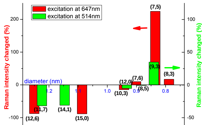
Figure 4. Relative SWNT population change by using PmPV 8 . The plot is constructed by using Raman intensity change for each SWNT shown in Figure 3.
