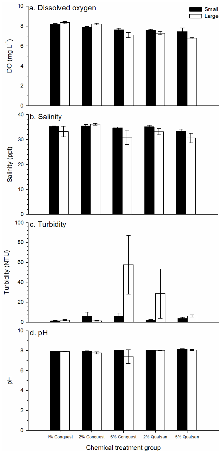
Figure 13. Baseline water quality data (mean \pm 1SE ) for (a) dissolved oxygen, (b) salinity, (c) turbidity, and (d) pH recorded at the commencement of chemical treatment trials, just prior to the addition of treatment chemical solutions.
