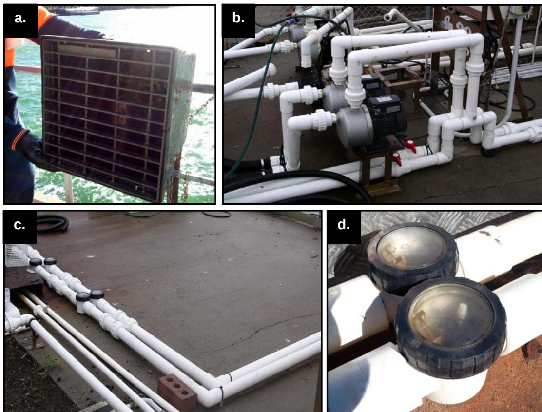
Figure 1. Elements of the purpose-built experimental sea water system, including (a) the grated sea chest, (b) pumps providing sea water, (c) 50 mm PVC piping comprising the pipework of the systems, and (d) two of the in-line screw-top access ports into which test mussels were placed for dosing
