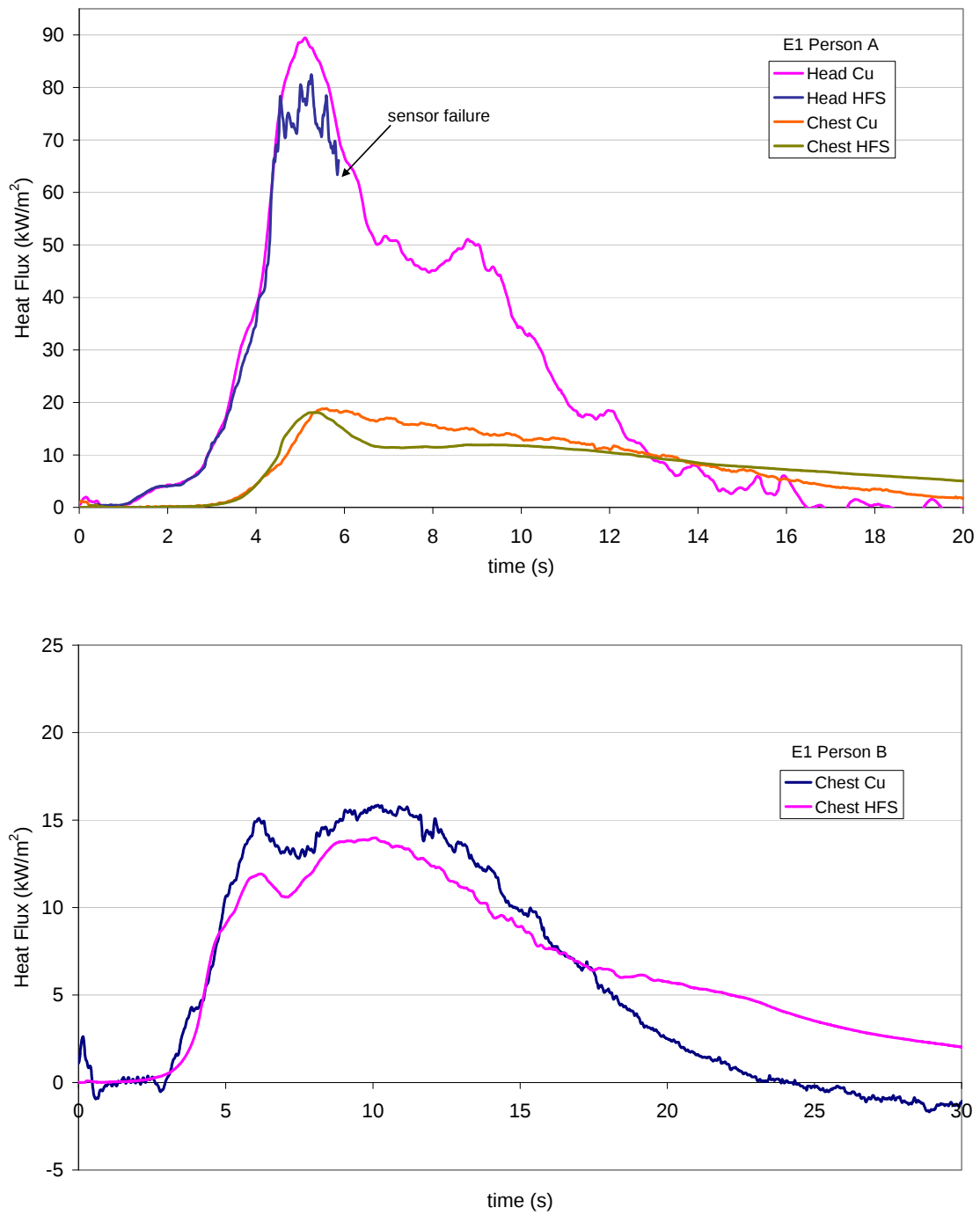
Figure 64: Omega HS-4 (HFS) and copper disc (Cu) heat flux measurement comparison for Experiment 1
