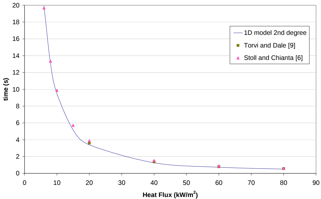
Figure 4: Comparison between the developed model and results from other workers for time to 2 nd degree burns when exposed to a constant heat flux
