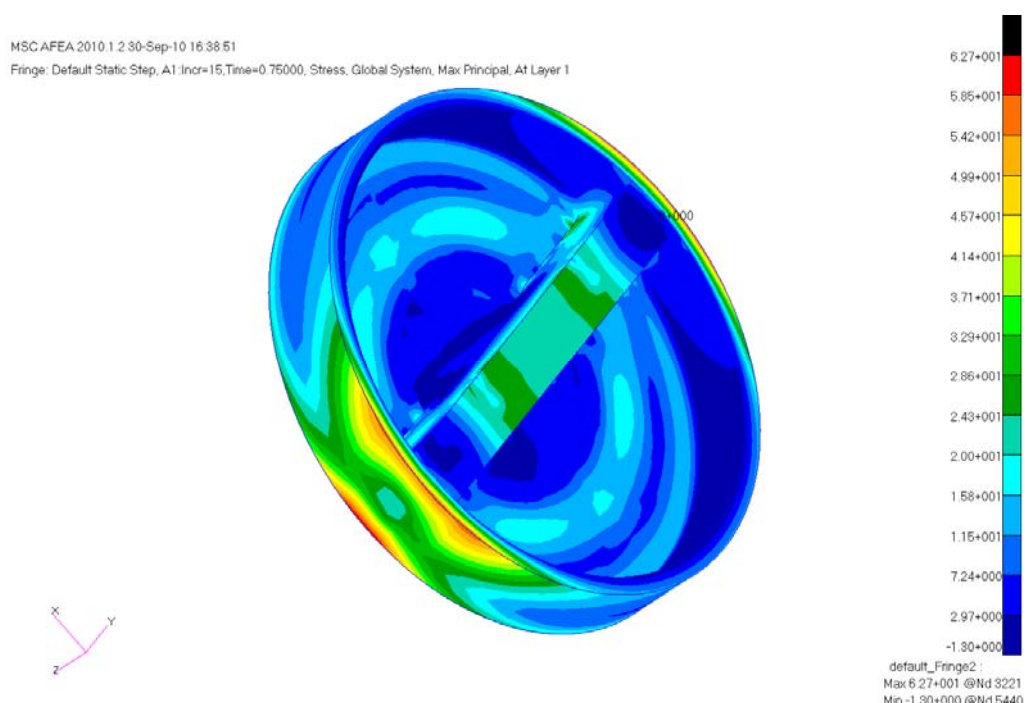
Figure 19: 1 st principal stress of polycarbonate end-cap of 62.7 MPa at 750 kPag internal pressure. Colour chart in MPa.
