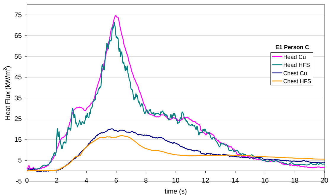
Figure 64: Omega HS-4 (HFS) and copper disc (Cu) heat flux measurement comparison for Experiment 1, (cont.)
