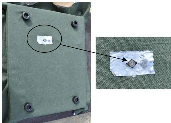
Figure 23: LE-080-250PSIA pressure transducer mounting arrangement for the chest and back
