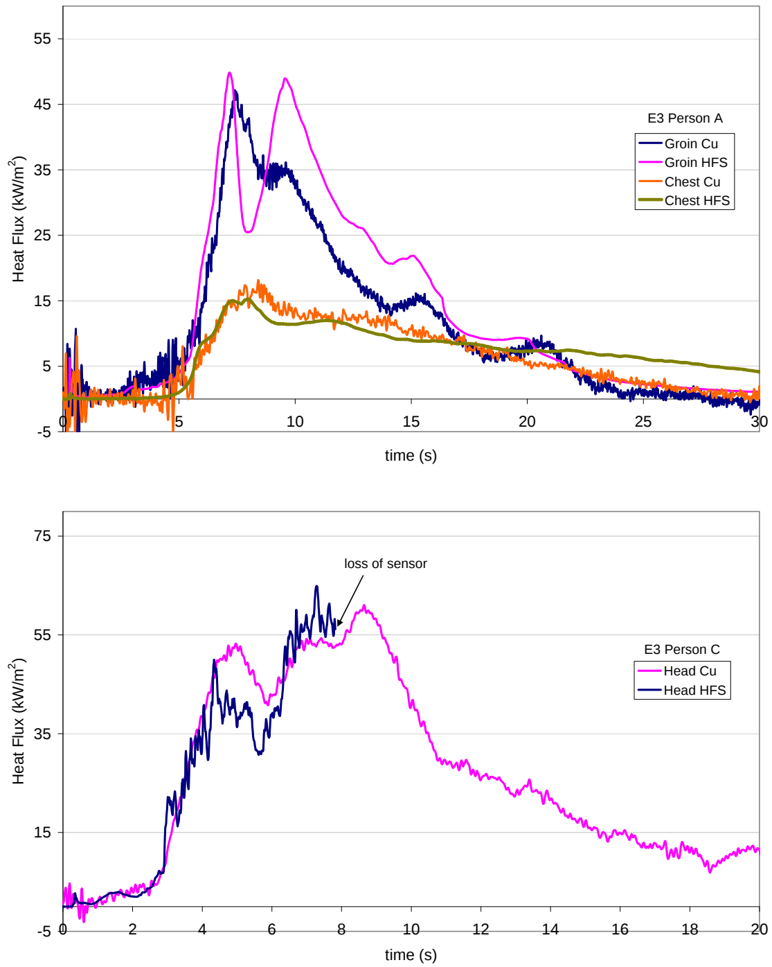
Figure 66: Omega HS-4 (HFS) and copper disc (Cu) heat flux measurement comparison for Experiment 3
