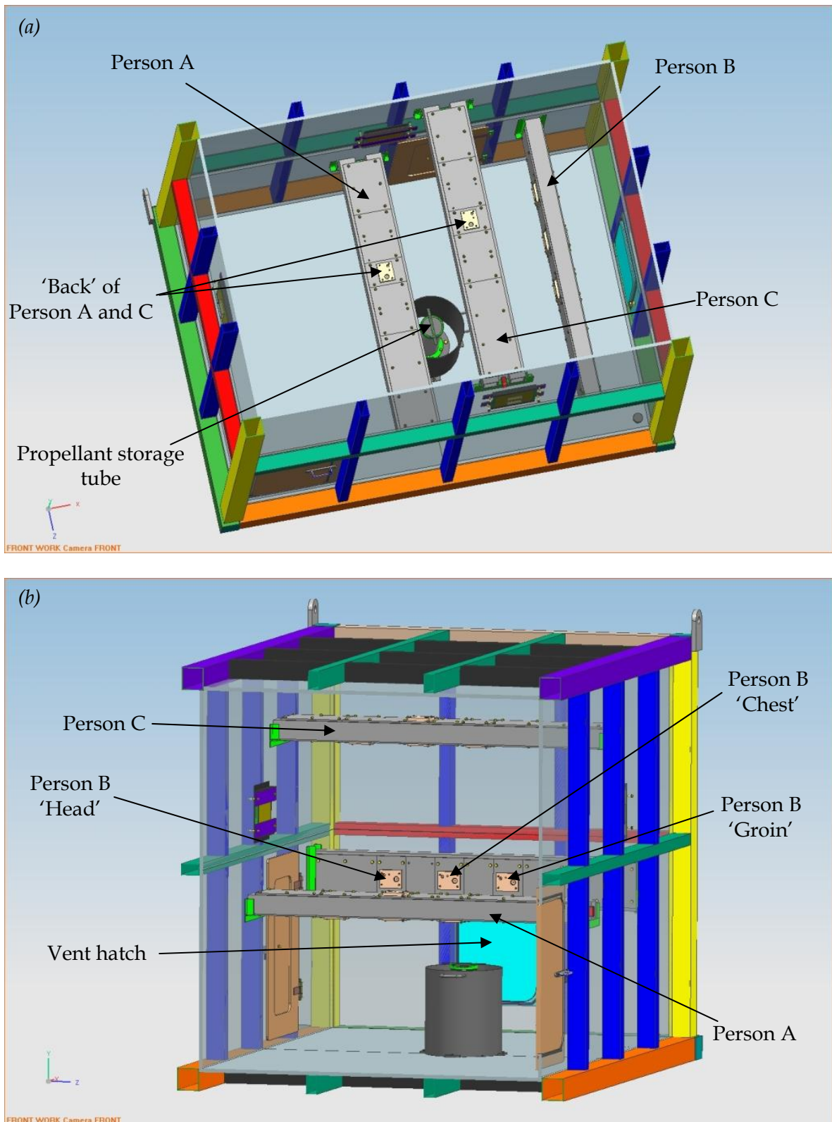
Figure 14: Schematic of the position of the three simulated personnel within the crew compartment and their respective groin, chest, back and head positions from (a) above, (b) end view
