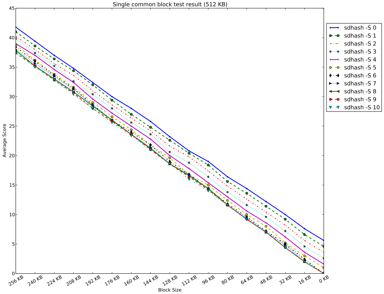
Figure 4.8: Average similarity scores for comparison of randomly generated 512-KiB files with a single common block of decreasing size, measured using sd score scale values between 0 and 10
