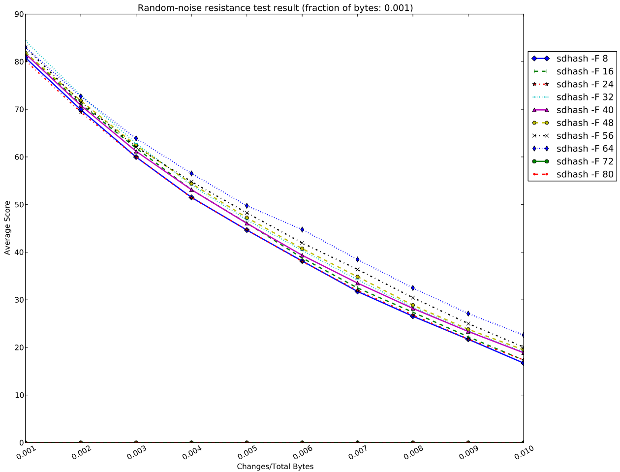
Figure 4.20: Average similarity scores for comparison of files against copies of themselves that are transformed with random byte insertions, deletions and substitutions, measured using popularity threshold values between 8 and 80 (number of transformations = \frac{1}{1000} of total bytes in original file). sdhash -F 16 matches Roussev's settings. sdhash -F 72 and sdhash -F 80 are flush with the x axis.
