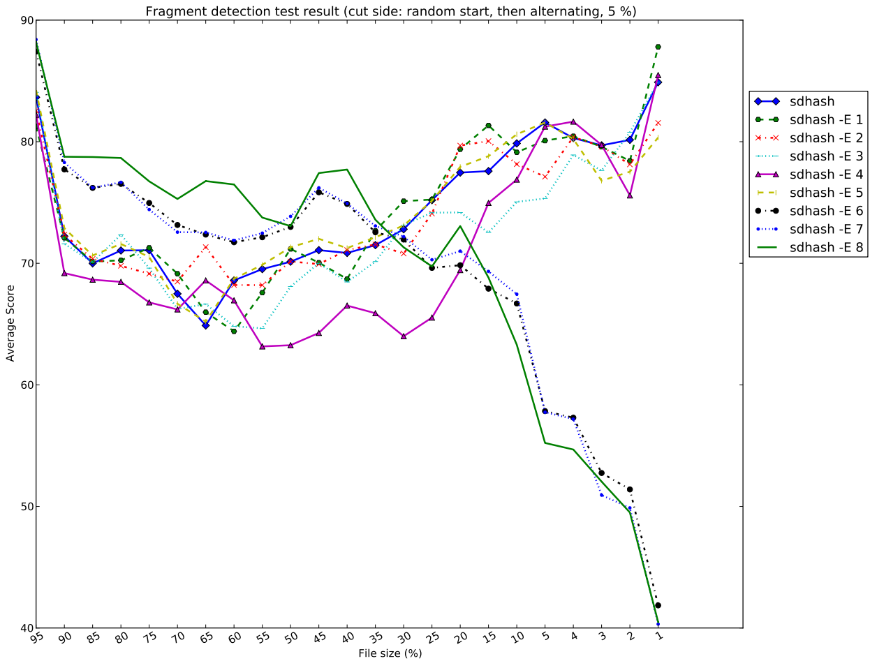
Figure 4.39: Average similarity scores for comparison of files against copies of themselves with slices removed from alternating ends, measured using 9 distinct entropy rank tables (slice size = 5% of file size until 5% remains, then 1%). sdbash uses Roussev’s settings.
