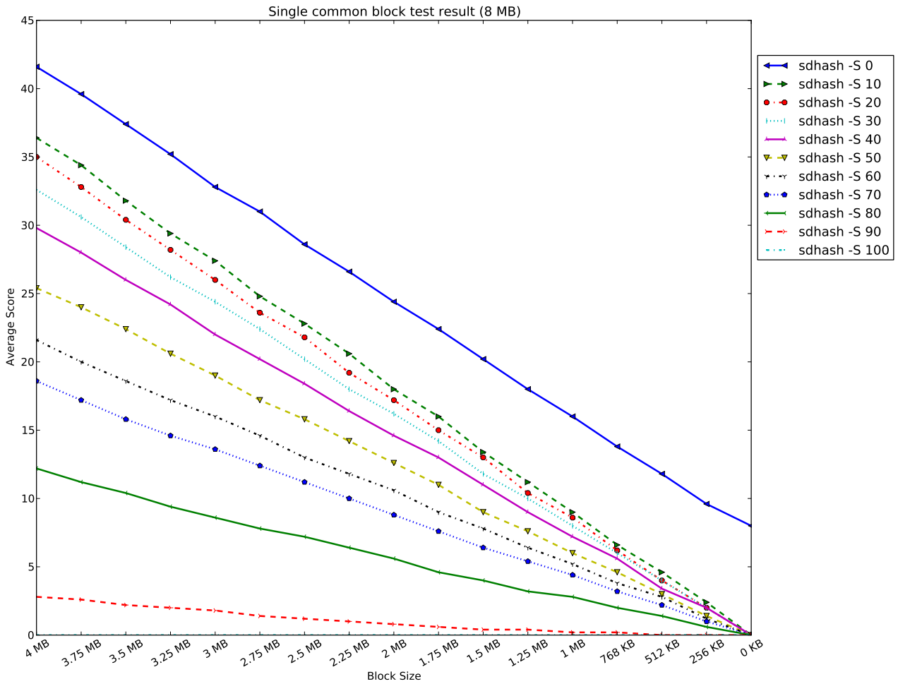
Figure 4.7: Average similarity scores for comparison of randomly generated 8-MiB files with a single common block of decreasing size, measured using sd score scale values between 0 and 100. sdhash -S 30 matches Roussev’s settings. sdhash -S 100 is flush with the x axis.
