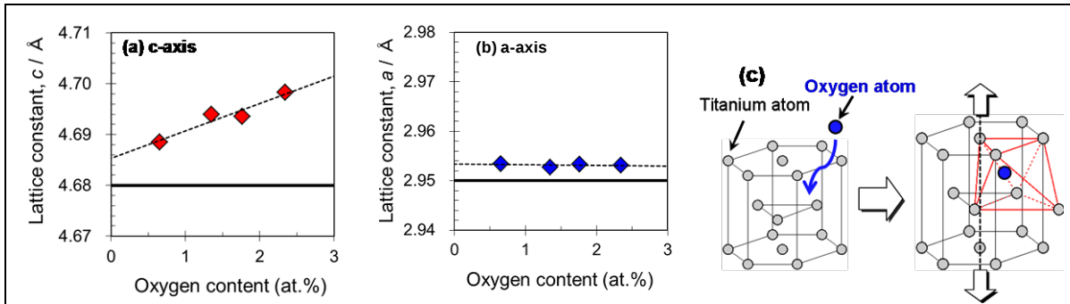
Figure 3. Dependence of lattice constant in c-axis (a) and a-axis (b) on oxygen content of extruded pure Ti powder materials with various TiO 2 particles; (c) oxygen atom is soluted between Ti atoms and the lattice spreads out in the c-axis direction.
