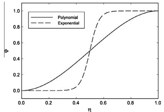
Fig. 1. Phase-field interfacial interpolation functions (2.17) and (2.18).
