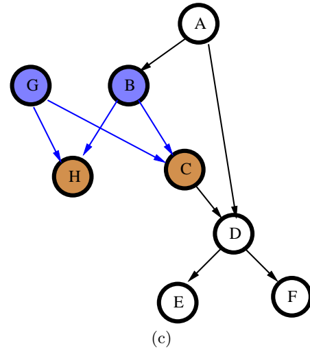
Figure 3: An example of how an update of the relations graph works: (a) shows the current relations graph consists of candidate solutions A through F; (b) two of these “old” candidates are shown to the user as well as two new ones, G and H, of which the user selects B and G; (c) based on the user’s selection, the relations graph is now updated.
