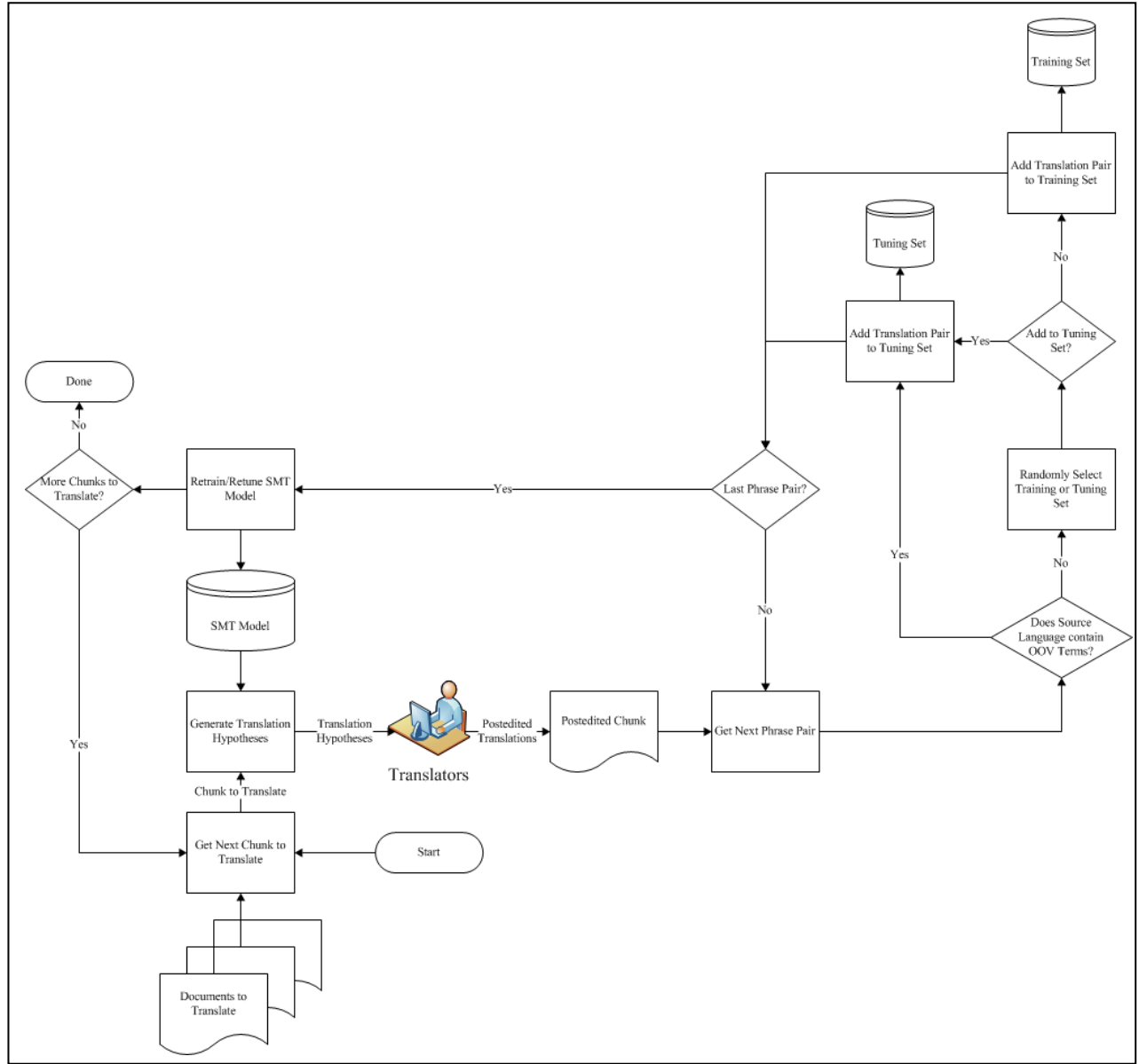
Figure 1. Iterative post-editing domain adaptation data flow.
