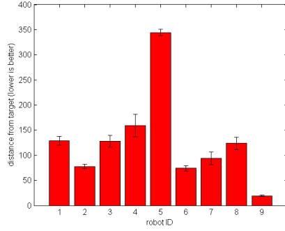
Figure 1: Robot fitness for nine sample robots. Error bars show the standard deviation in fitness for the thirty runs.
