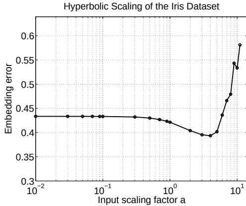
Figure 8. The effect of scaling of the dissimilarities on the embedding error for the Iris Dataset (Anderson 1935). The input dissimilarities are the Euclidean distances between pairs of original points. This MDS-PD result reveals that the Iris dataset is better suited for embedding to the hyperbolic plane than to the Euclidean plane.
