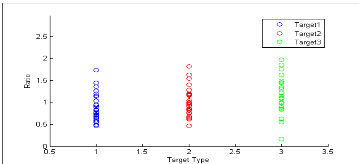
Figure 5. Feature values (average amplitude and maxium peak over trough) for targets 1, 2, and 3.
