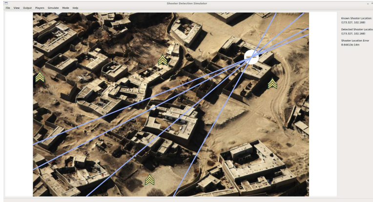
Figure 6. Our GUI after performing shooter detection in an error-free case. The purple lines show the major axes of each of the four conics containing a subset of three of the microphones. We see that the shooter (gun symbol) has changed to a bullet, indicating the detected position. The detected position and detection error are displayed in the right-hand information bar.
