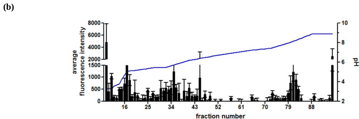
Figure 6.2. PCNA Isoform Separation as Determined by Reverse-Phase Immunological Assay. Chromatin-bound MCF7 breast cancer cell nuclear lysate was fractionated by free flow electrophoresis and the fractions were dot blotted onto a piece of PVDF membrane. A reverse-phase immunological assay was performed using a PC10 monoclonal total PCNA antibody and a fluorescently-labeled secondary antibody reporter. (a) Membrane was imaged using a Typhoon Trio+ image scanner using an excitation of 488nm and an emission of 526nm. Individual pixel intensities from each spot of protein deposition were averaged. (b) The average intensity of each spot deposition versus fraction number and pH. These demonstrate four different populations of PCNA isoforms.
