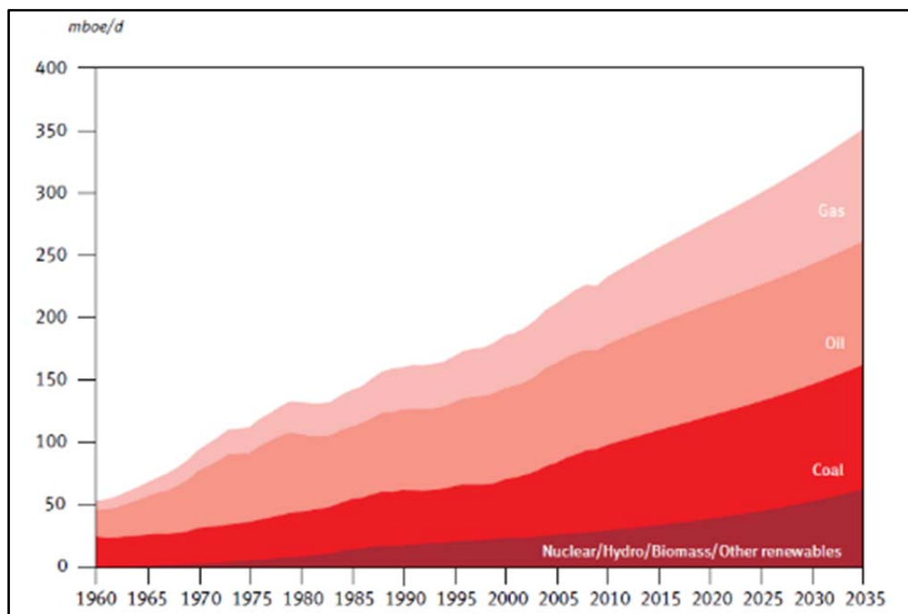
Figure 8. World Supply of Primary Energy by Fuel Type (OPEC, 2011)
