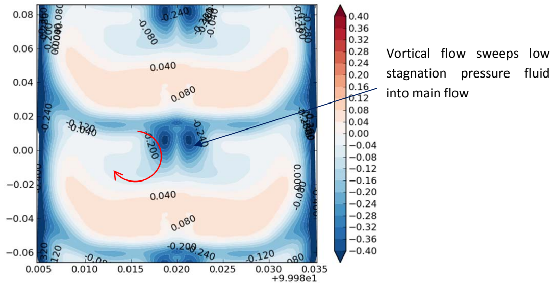
Figure 4 Exit stagnation pressure coefficient predicted by TurboStream for datum blade with a steady jet at inlet.
