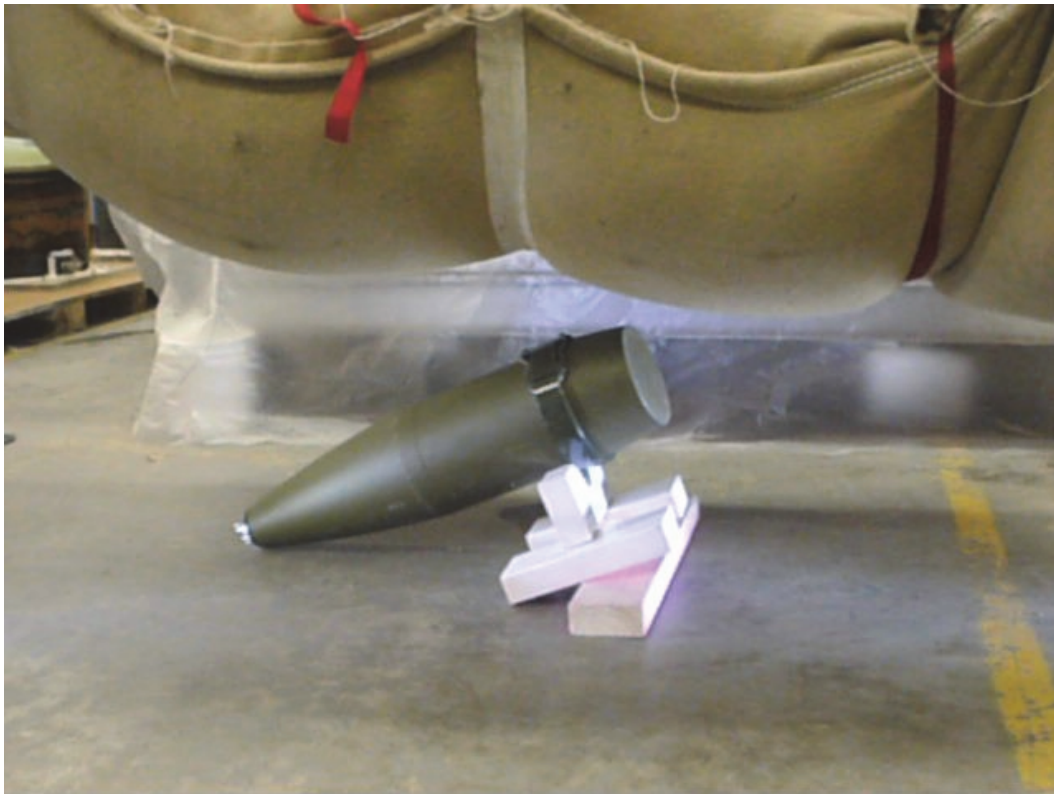
Figure 18. 155mm M107 in elevation jig.
