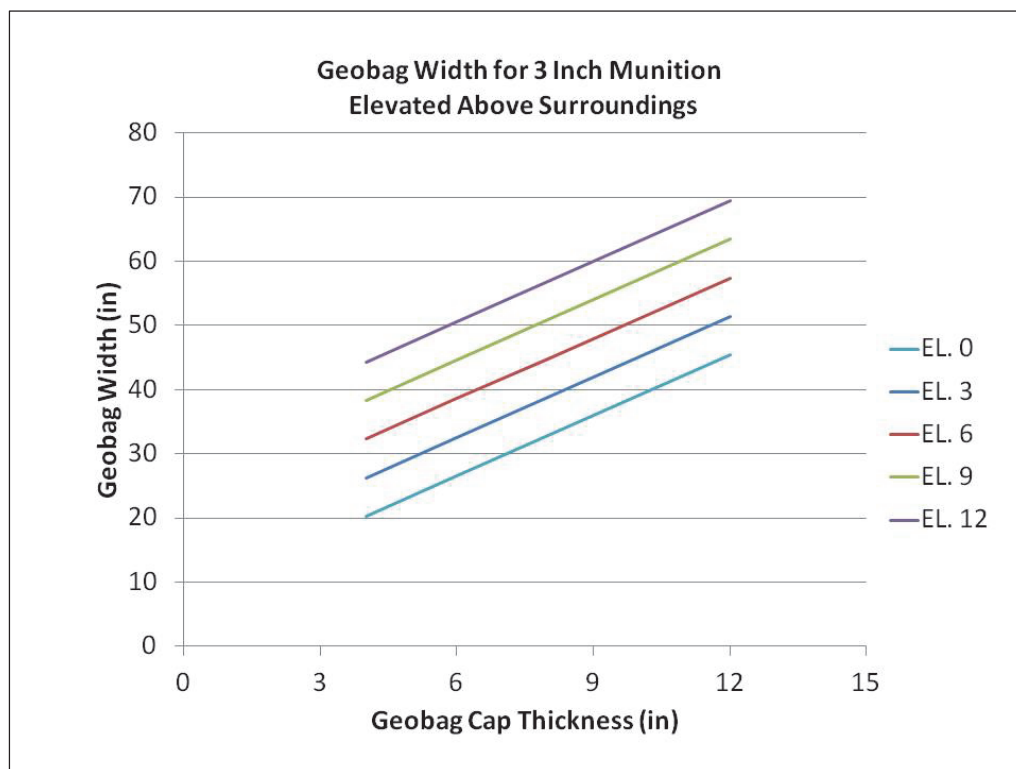
Figure 37. Geobag sizing guidance for 3 inch diameter or equivalent munitions.
