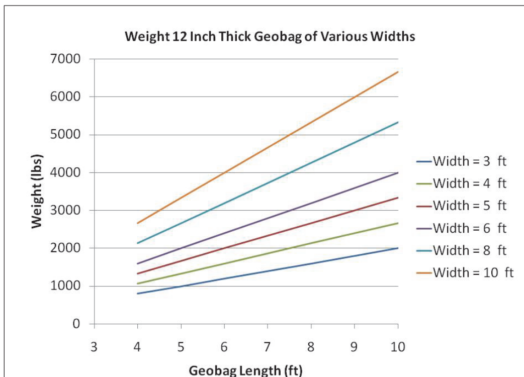
Figure 35. Weight of geobags with 12 in thicknesses.
