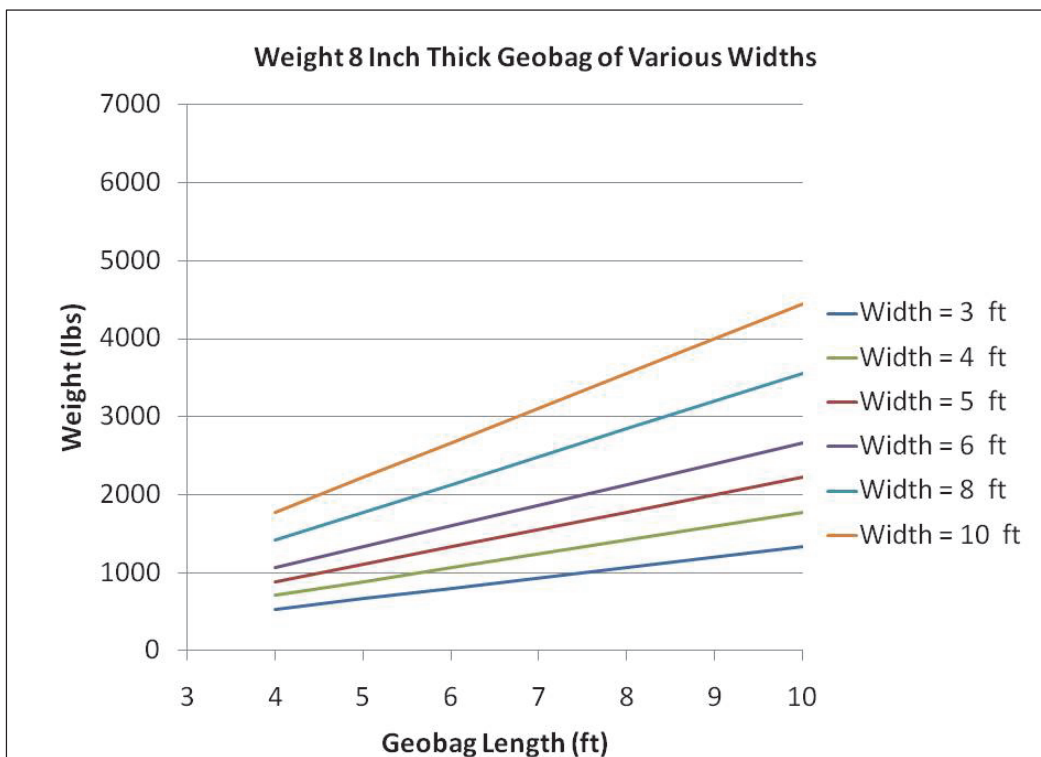
Figure 33. Weight of geobags with 8 inch thicknesses.
