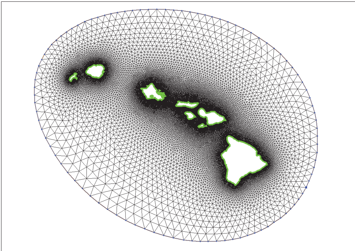
Figure 7. Hawaiian Island ADCIRC grid.
