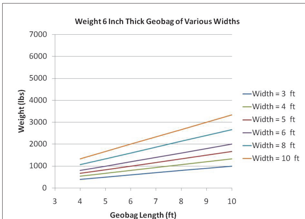
Figure 32. Weight of geobags with 6 inch thicknesses.
