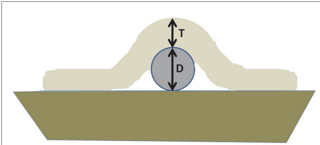
Figure 36. Geobag sizing information.
