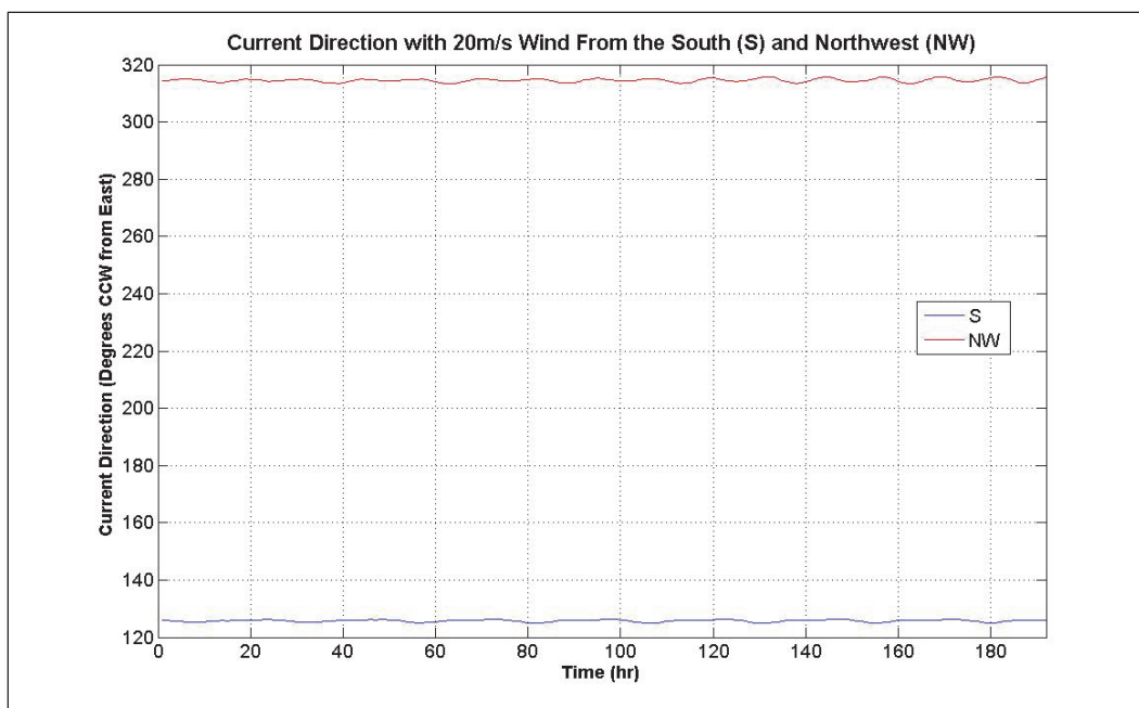
Figure 14. Tidal current direction with steady 20 m/s wind forcing.
