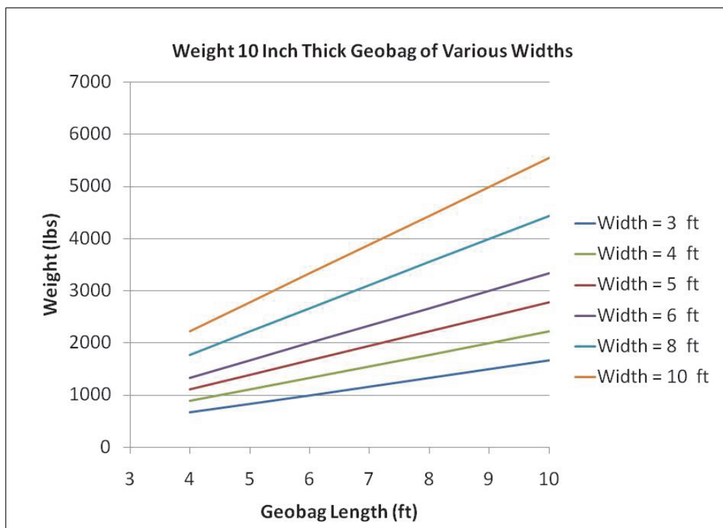
Figure 34. Weight of geobags with 10 inch thicknesses.
