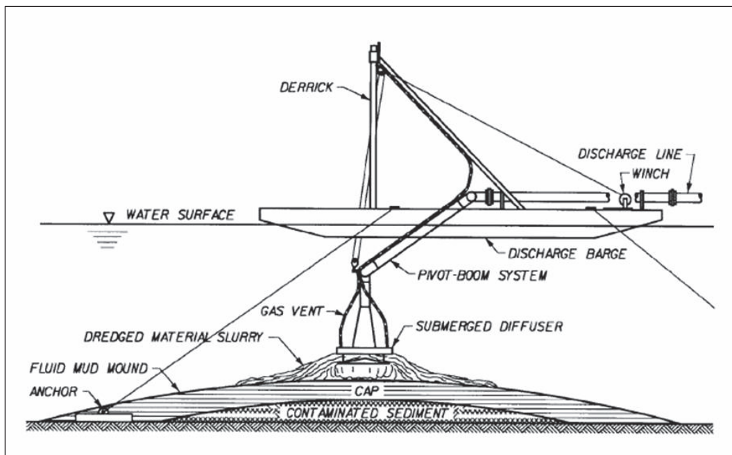
Figure 1. Cap placement technique for covering contaminated sediments.
