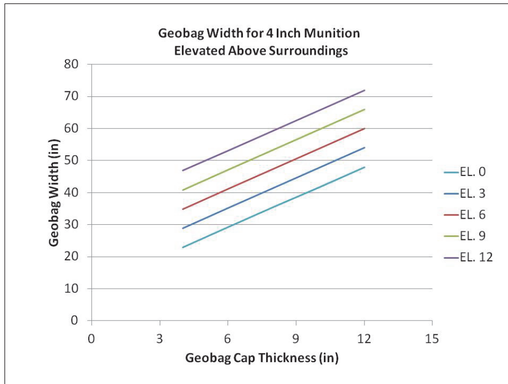
Figure 38. Geobag sizing guidance for 4 inch diameter or equivalent munitions.
