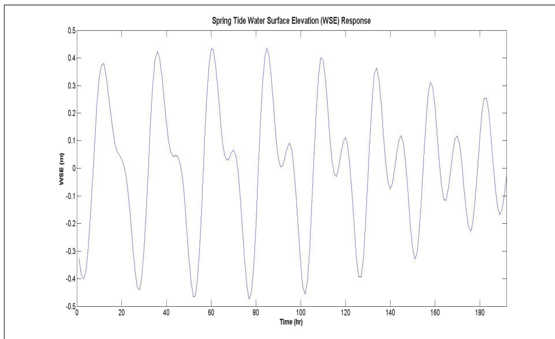
Figure 10. Predicted water surface elevation without wind forcing.
