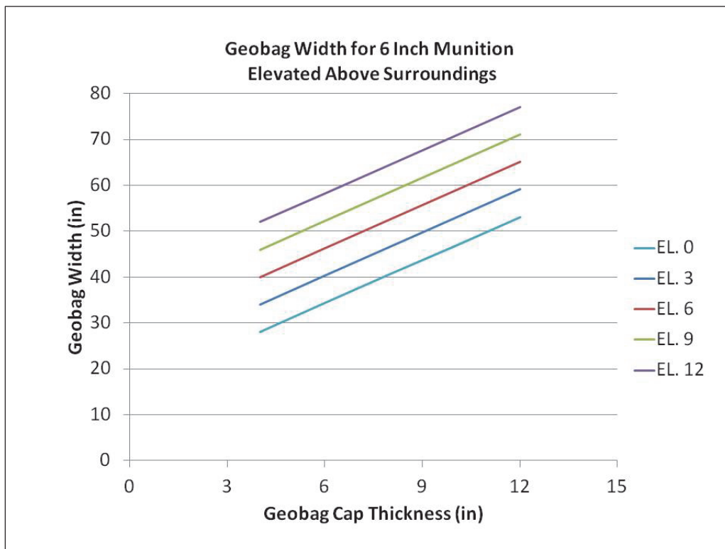
Figure 39. Geobag sizing guidance for 6 in diameter or equivalent munitions.
