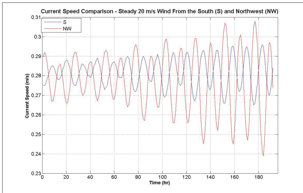
Figure 12. Comparison of tidal current speeds with 20 m/s wind forcing.
