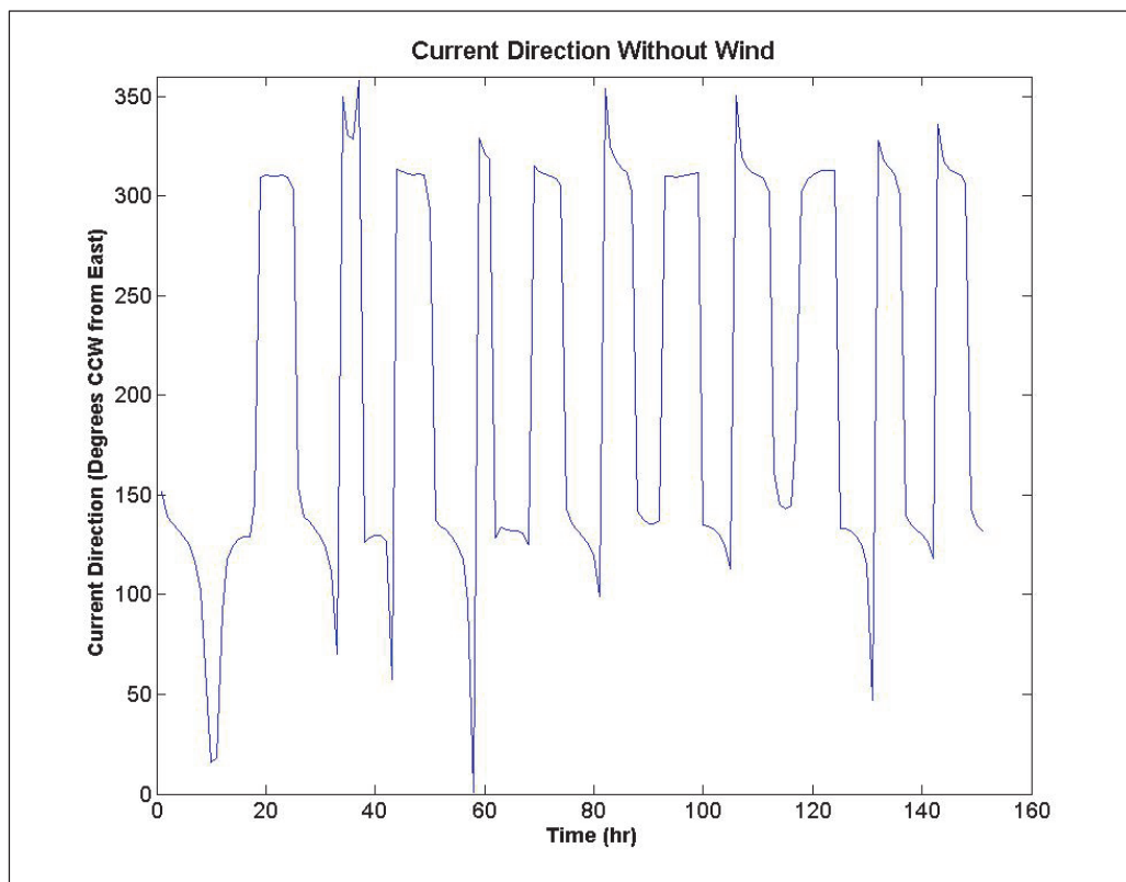
Figure 13. Tidal current direction without wind forcing.
