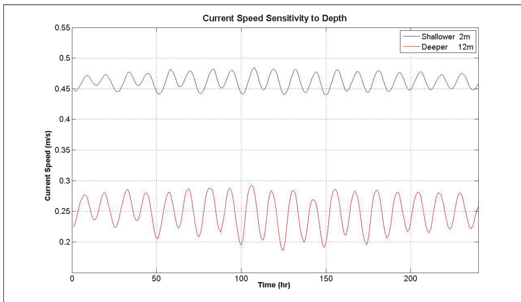
Figure 15. Cross-shore current variation with depth, steady 20 m/s wind forcing.
