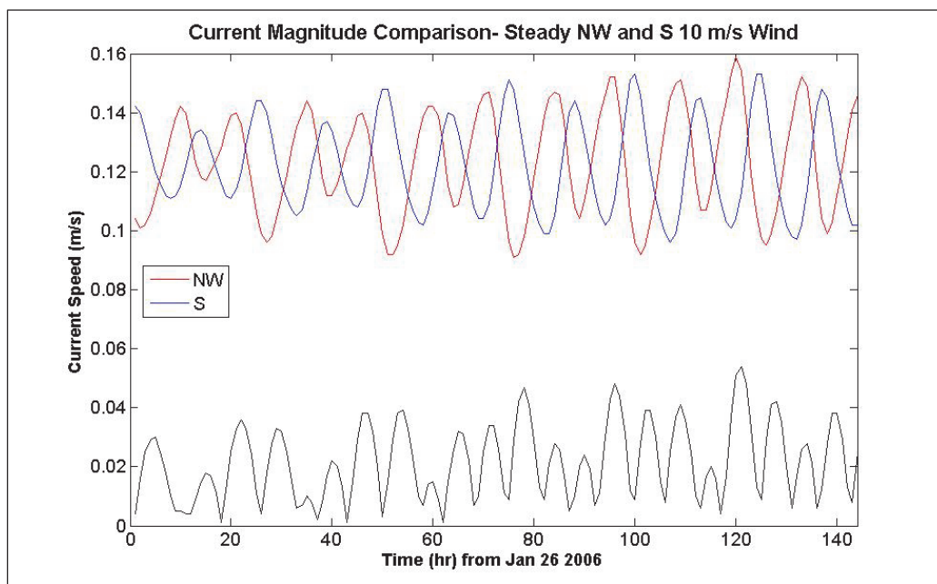
Figure 11. Comparison of tidal current speeds with and without wind forcing; the black line at the bottom represents the tide-forced current speed without wind forcing.
