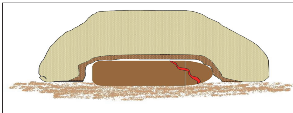
Figure 3. Cross-section of a geobag placed over underwater ordnance.
