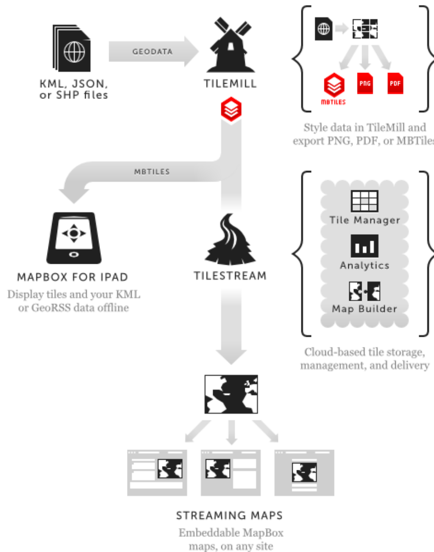
Figure 17. MapBox Architecture 145
