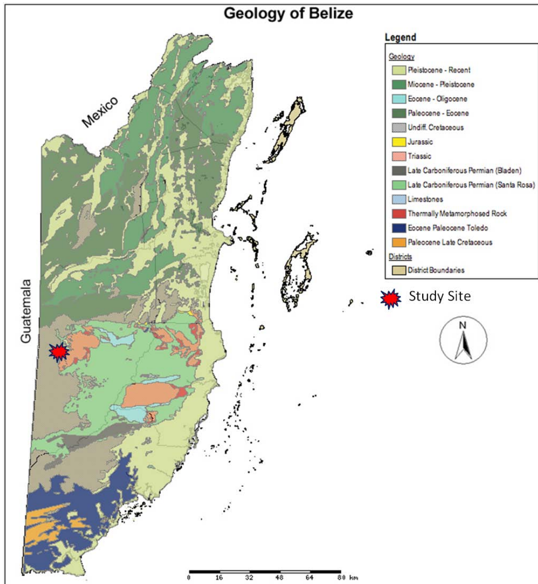
Figure 3: Belize's Geology
