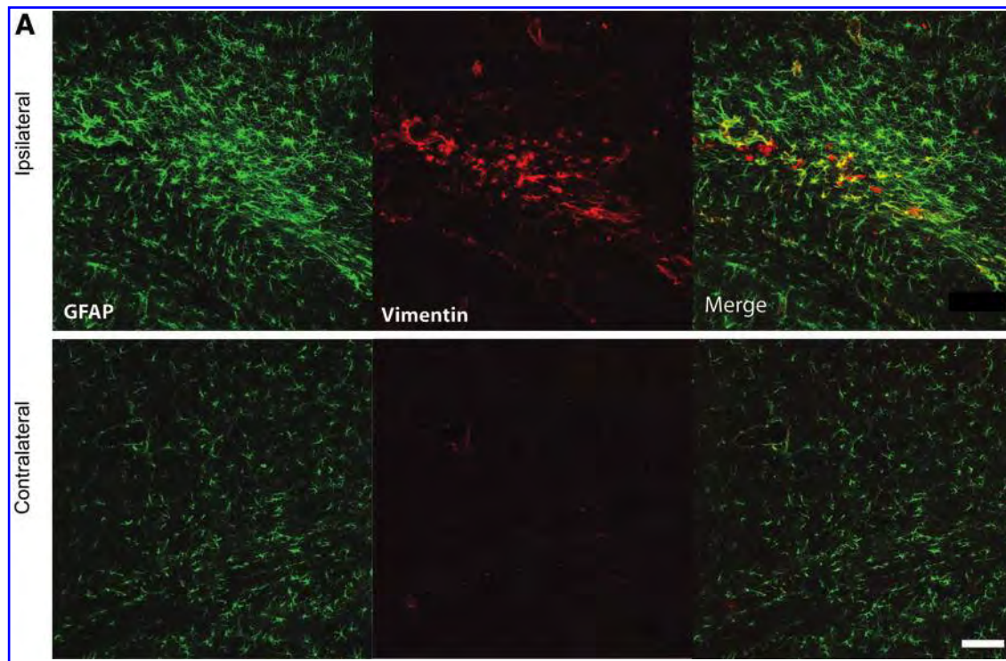
FIG. 5. Representative immunostaining 6h after 1-atm mFLP injury. Images of inflammatory activated astrocytes in ipsilateral parietal cortex, as indicated by GFAP + cells and colocalized (A) vimentin (scale bar = 50 microns). (B) Cortical astrocytic activation 18 days after mFLP injury, as indicated by GFAP immunostaining (original magnification, 20 \times ). Quantitation of cortical GFAP + cells 18 days after mFLP injury ( p < 0.05 ). Color image is available online at www.liebertpub.com/neu
