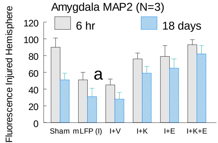
Figure 3. Quantitation of immunofluorescence 18 days after mLFP injury. (a) = p < 0.01 naïve or sham vs Injury or injury + vehicle (I+V); p < 0.05 Injury or I+V vs I+Kineret (I+K) or injury + Etanercept (I+E) or both (I+K+E); all other comparisons are not significant.
