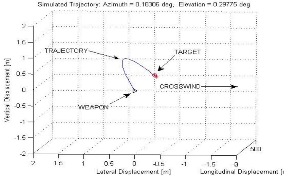
Figure 21. Simulated Trajectory
