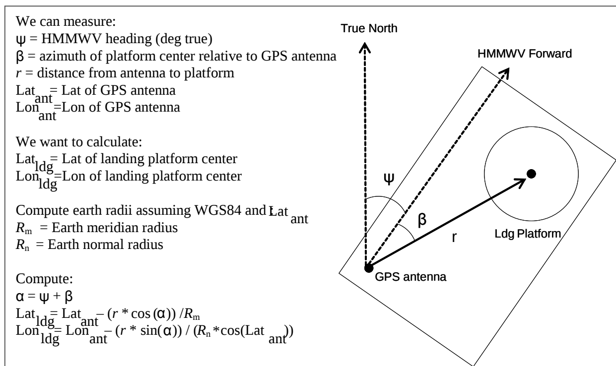
Figure 6. Offset Corrections
