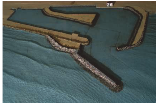
Figure 6. Ma'alaea Harbor, Maui, HI: coastal, fixed-bed, 3D model for studying effects of proposed improvements on harbor wave action, navigation and surfing conditions (Source: Ray Bottin).
