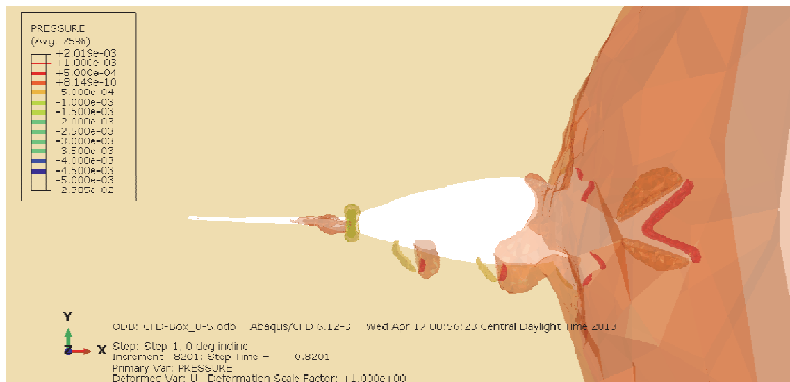
Figure 25. Pressure profile for fish moving along the flow direction at an angle of attack of 0 degrees.
